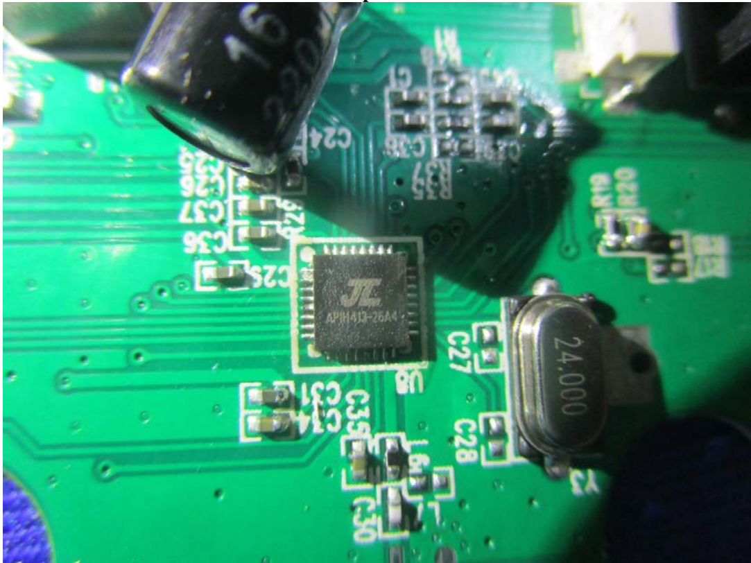
Chip View
