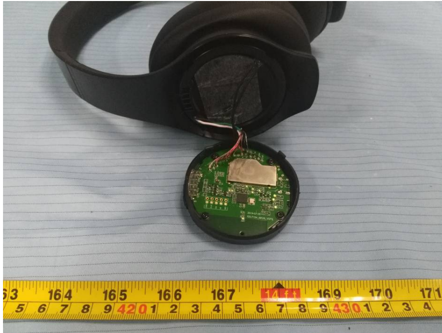
EUT – Left Ear Cover off View
