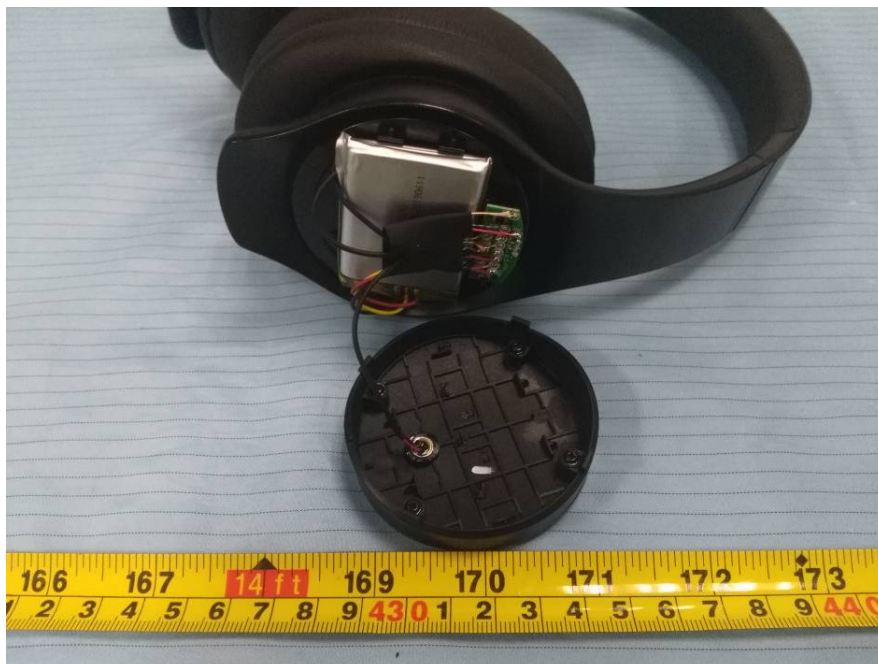
EUT – Right Ear Cover off View
