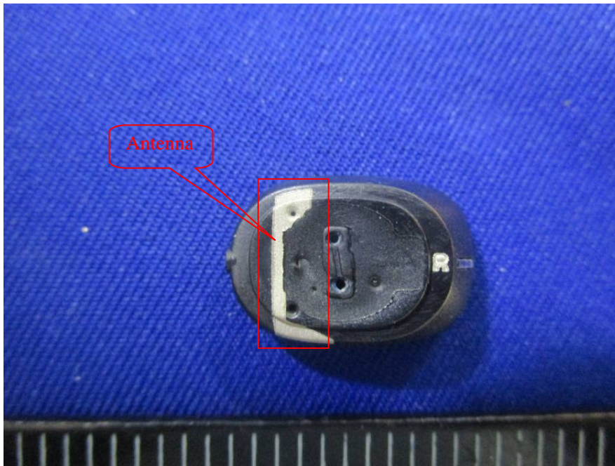
EUT – Right Earbud Antenna View
