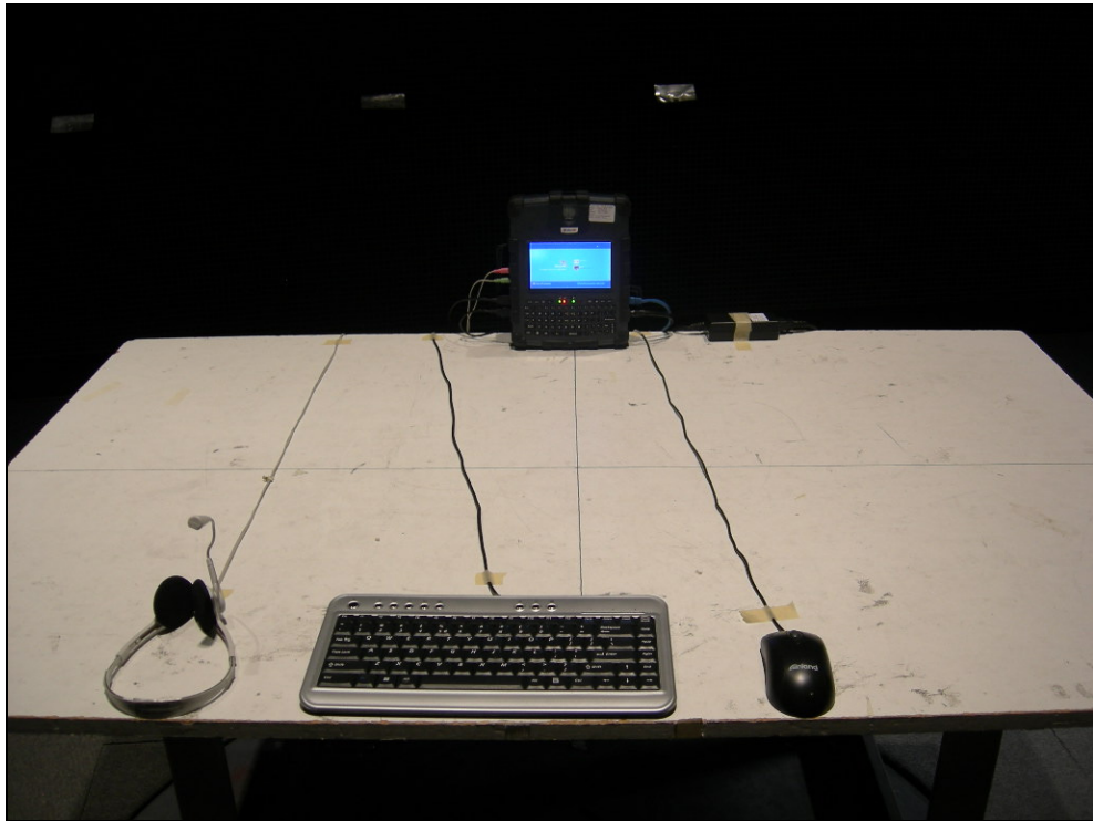
Figure 5: Radiated Emissions – Y Position
