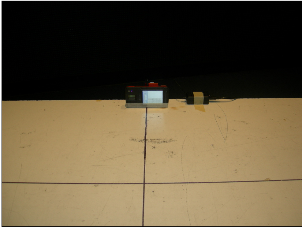
Figure 9: Test Setup – Radiated Emissions Z Position
