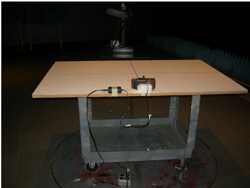
Figure 12: Test Setup – Radiated Emissions Z Position
