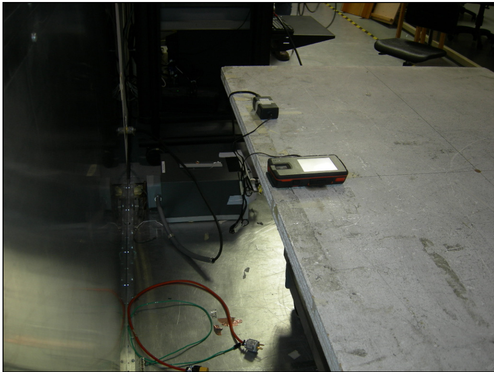
Figure 17: Test Setup – Conducted Emissions X Position
