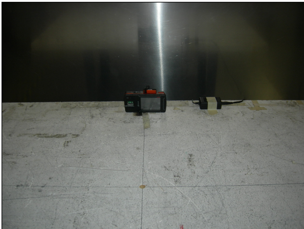
Figure 14: Test Setup – Conducted Emissions Z Position
