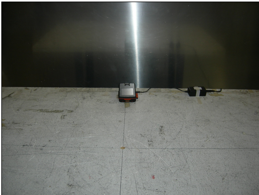
Figure 16: Test Setup – Conducted Emissions X Position
