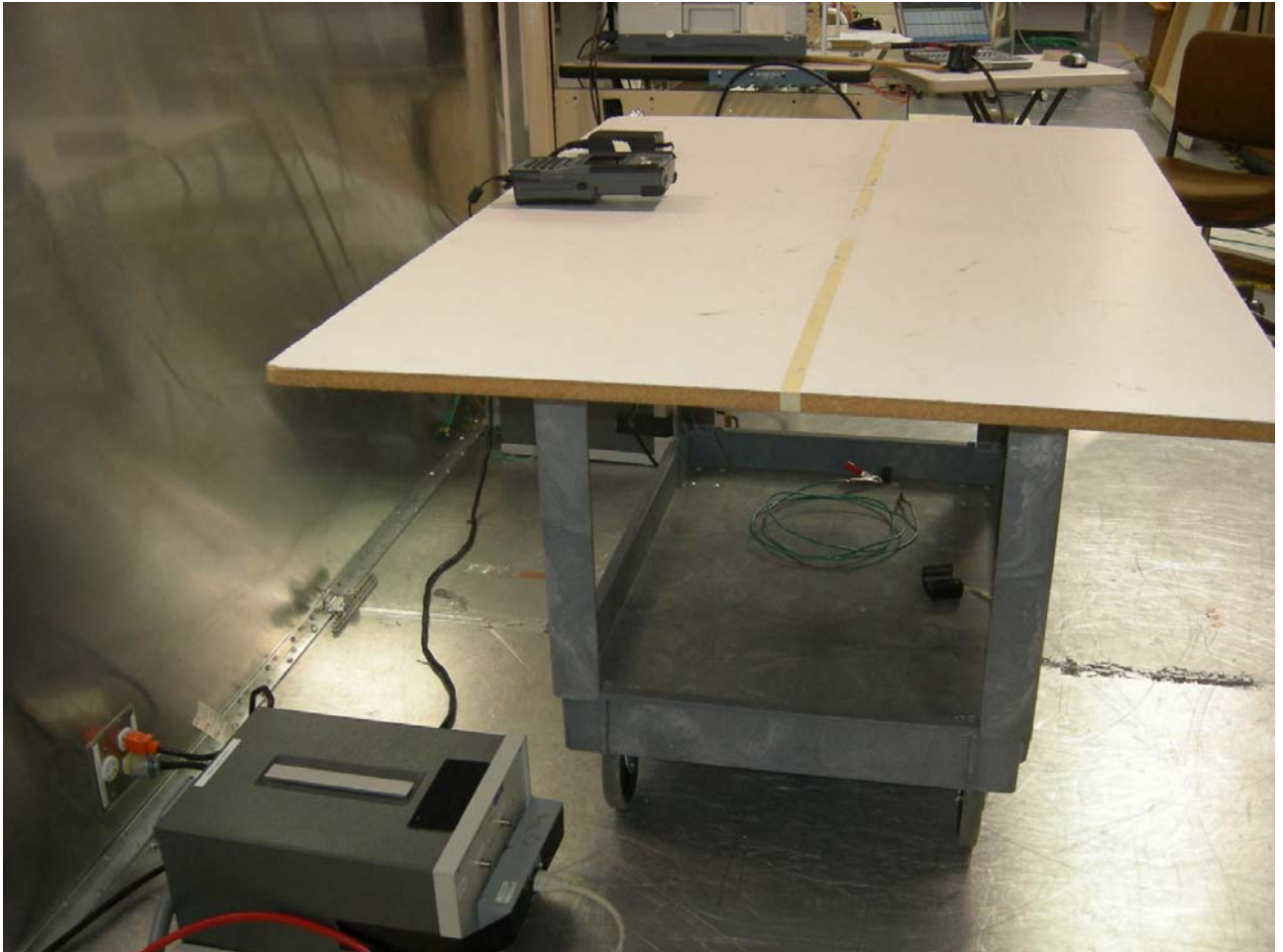
Figure 8: Conducted Emissions
