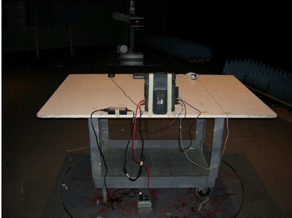
Figure 2: Radiated Emissions – Y Position
