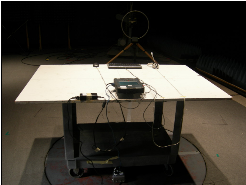
Figure 4: Radiated Emissions – X Position
