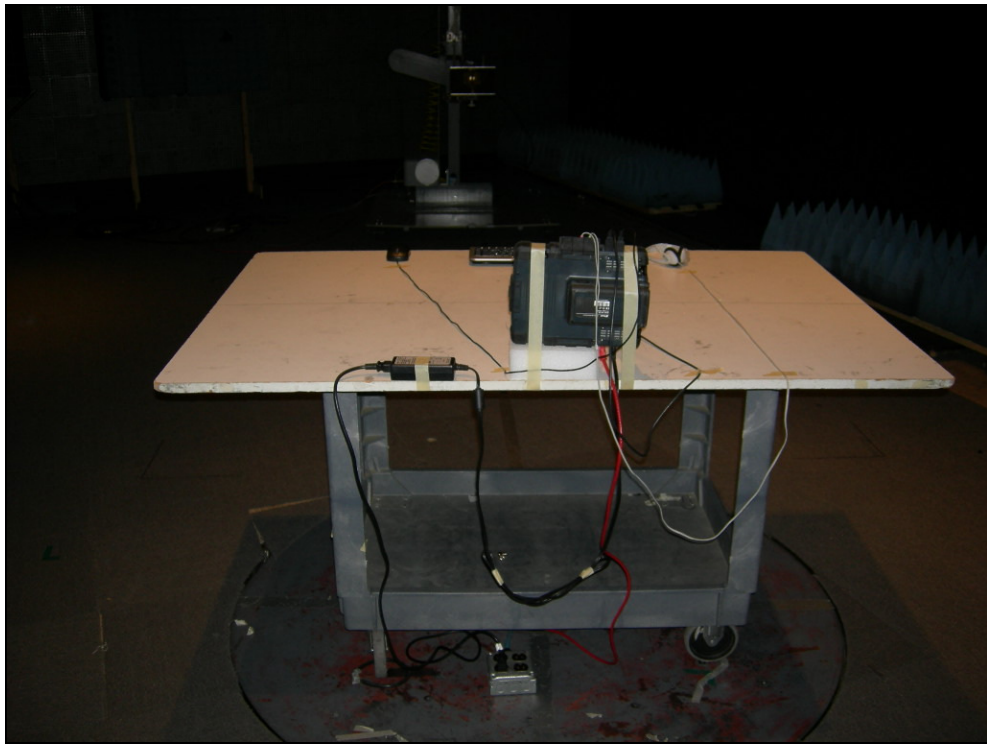
Figure 3: Radiated Emissions – Z Position
