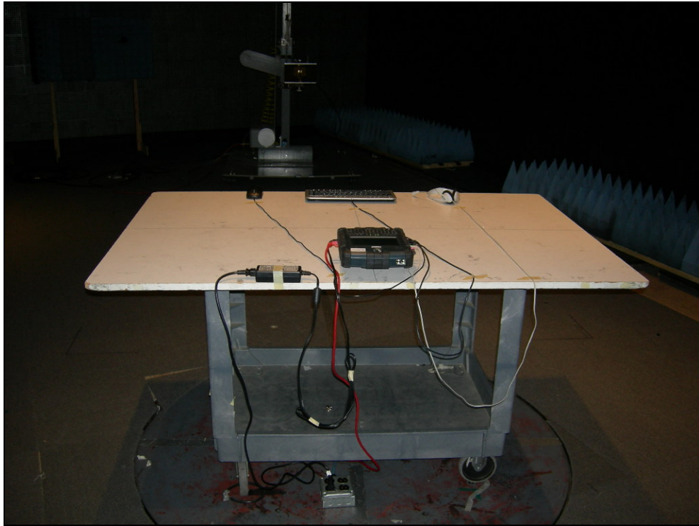
Figure 1: Radiated Emissions – X Position
