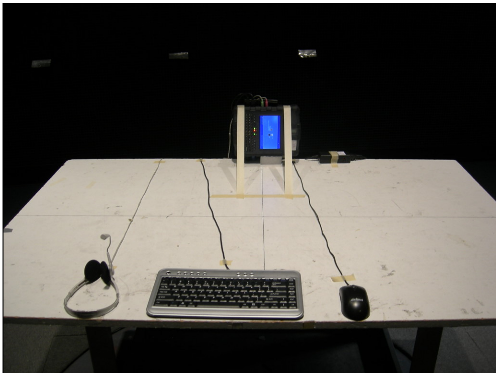
Figure 6: Radiated Emissions – Z Position
