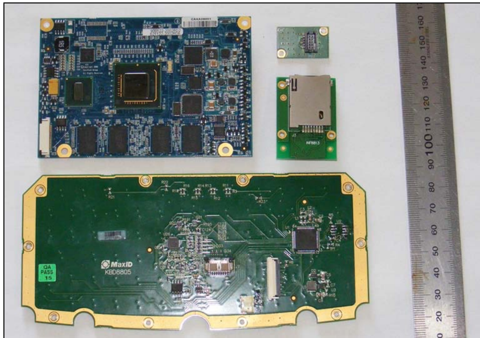
Figure 3: PCBs – Front
