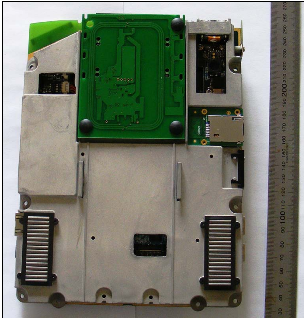
Figure 8: PCBs – Installed, Back (Battery Pack Removed)
