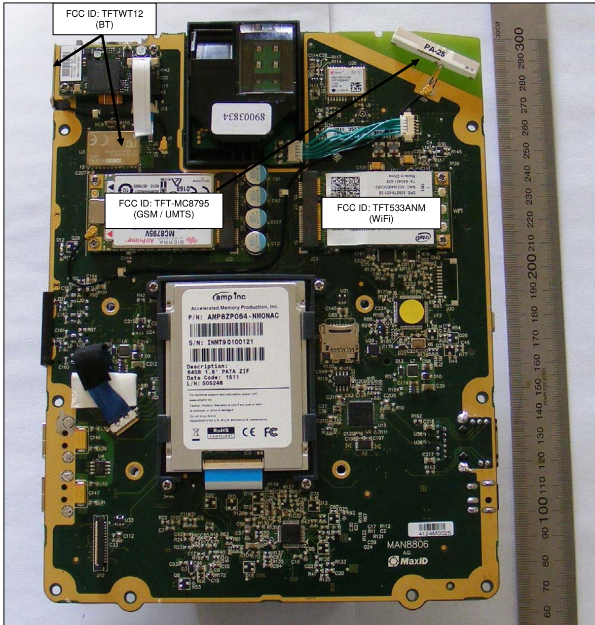
Figure 1: Main PCB - Front
