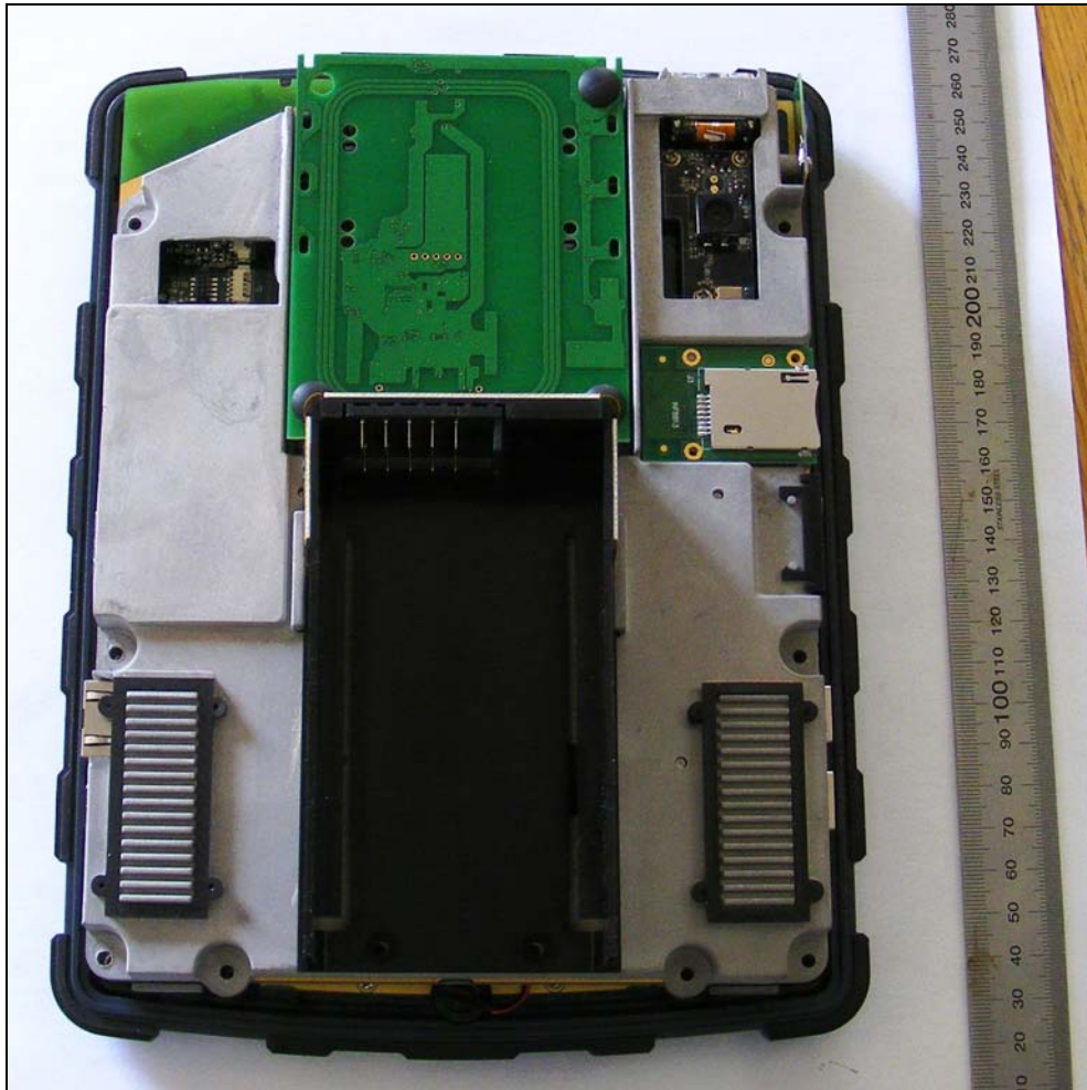
Figure 7: PCBs – Installed, Back
