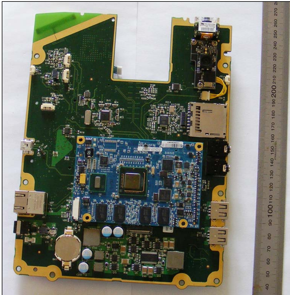
Figure 2: Main PCB - Back
