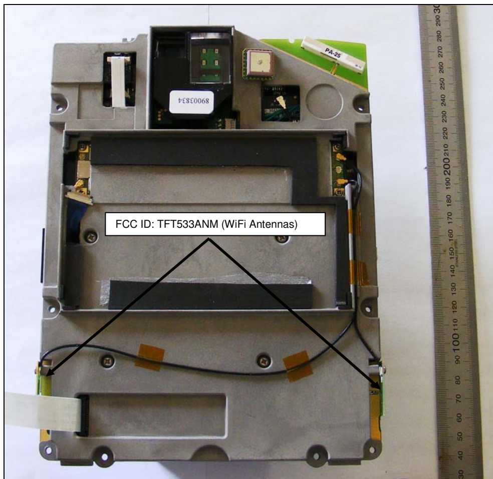
Figure 6: PCBs – Installed, Front (Screen Removed)
