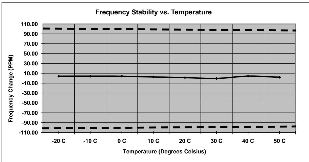
Figure 7.5.2-1: Frequency Stability
