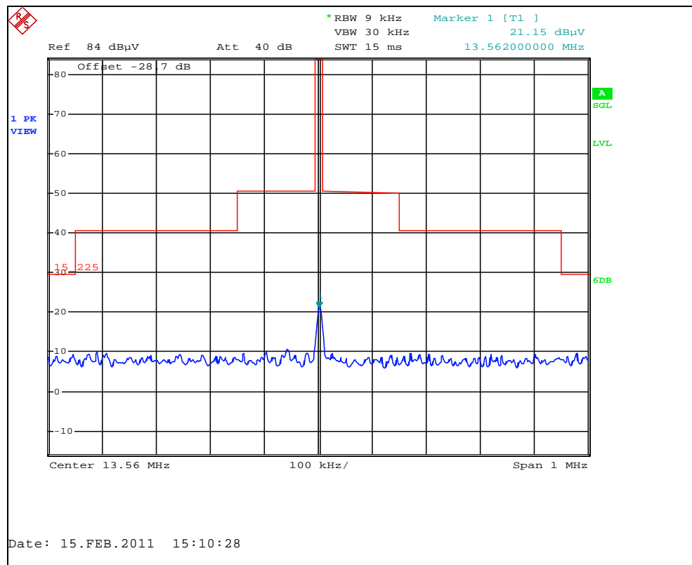
Figure 7.3.1.2-3: Emission Mask Plot – Z Orientation
