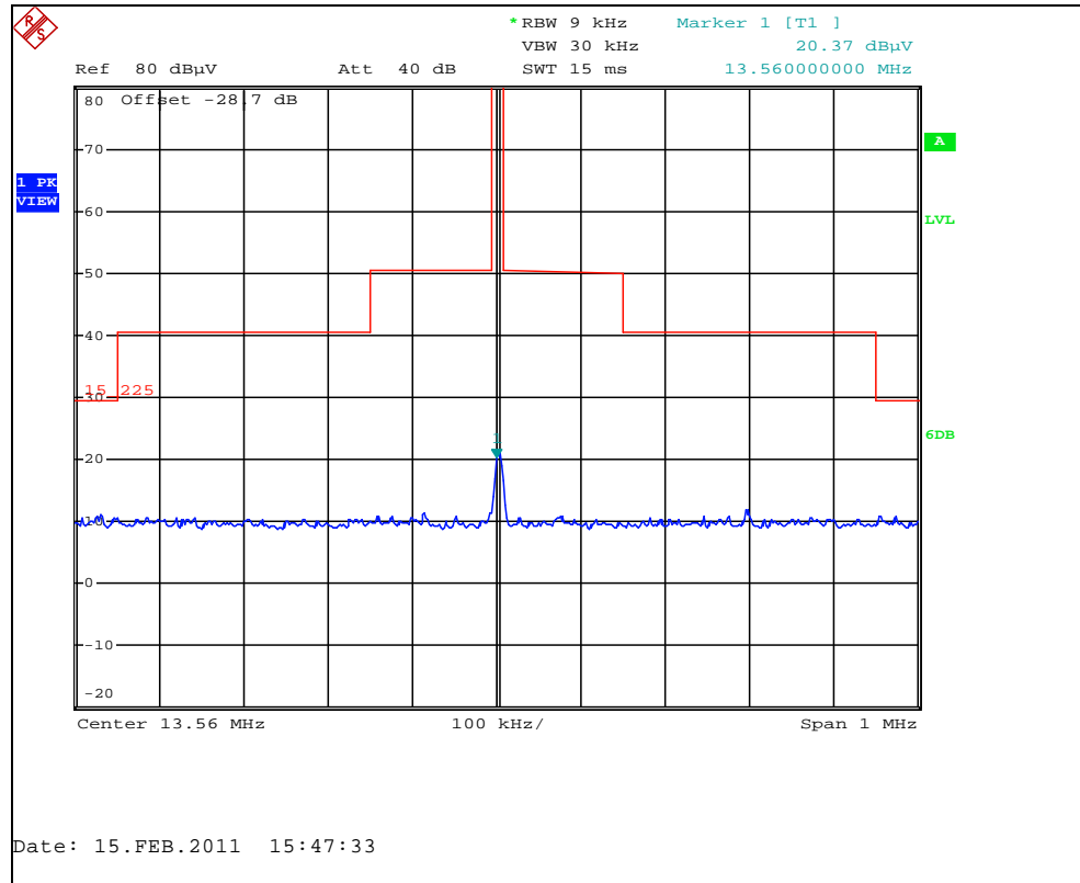
Figure 7.3.1.2-2: Emission Mask Plot – Y Orientation
