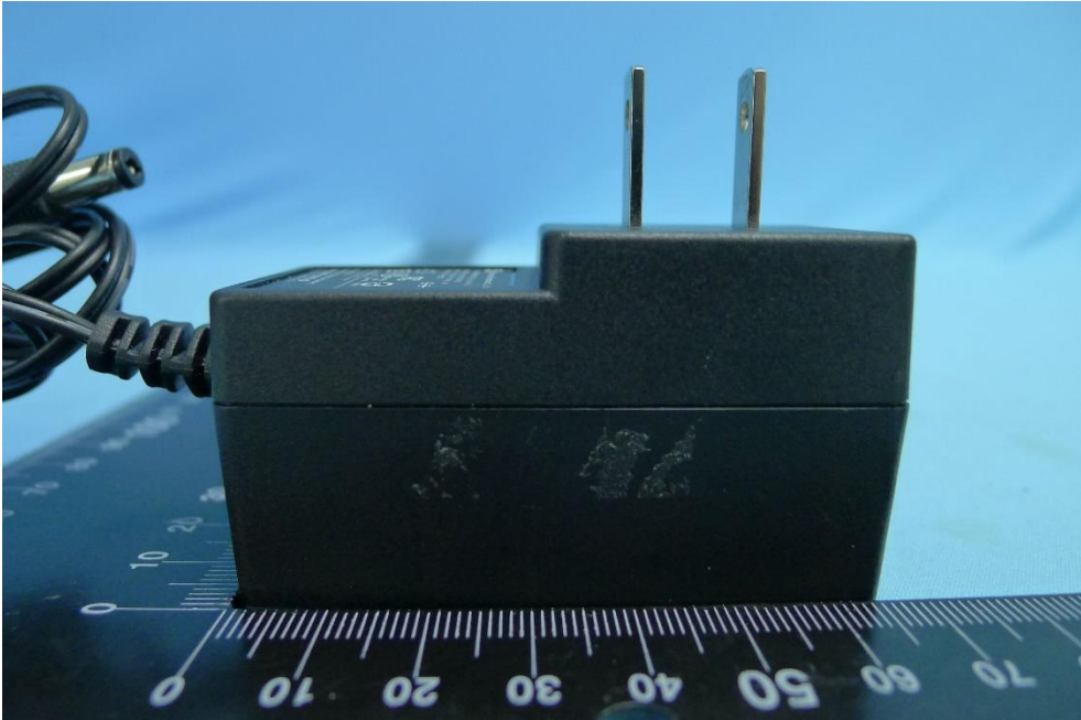
(19) Adapter (A106-2050130U)
