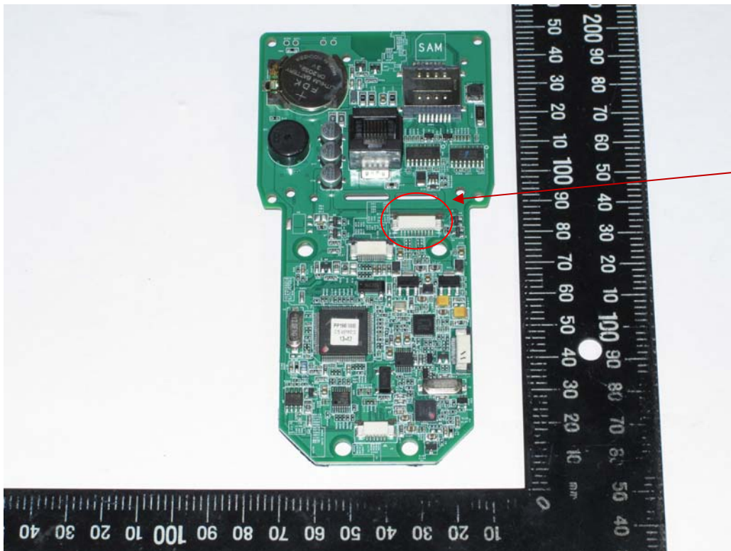
Antenna Connector
