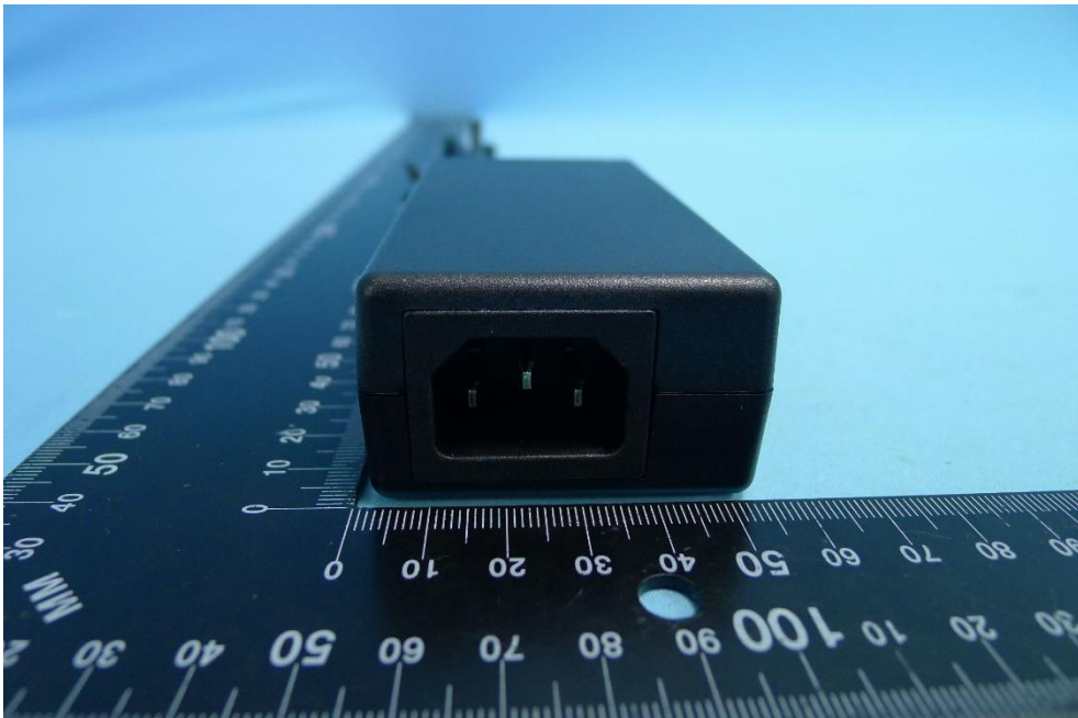
(24) Adapter (PA150-090T1A500)
