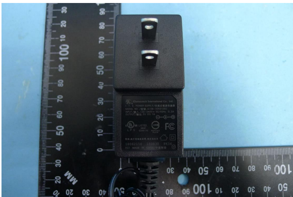
(12) EUT Photo (Adapter: A106-2050103U)
