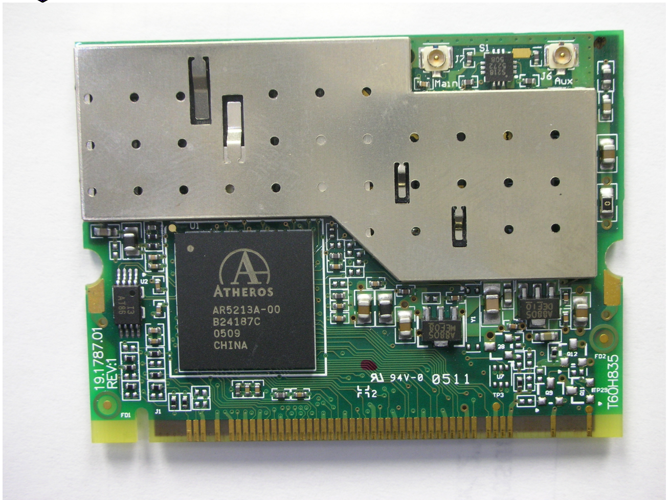
Front of FR100
