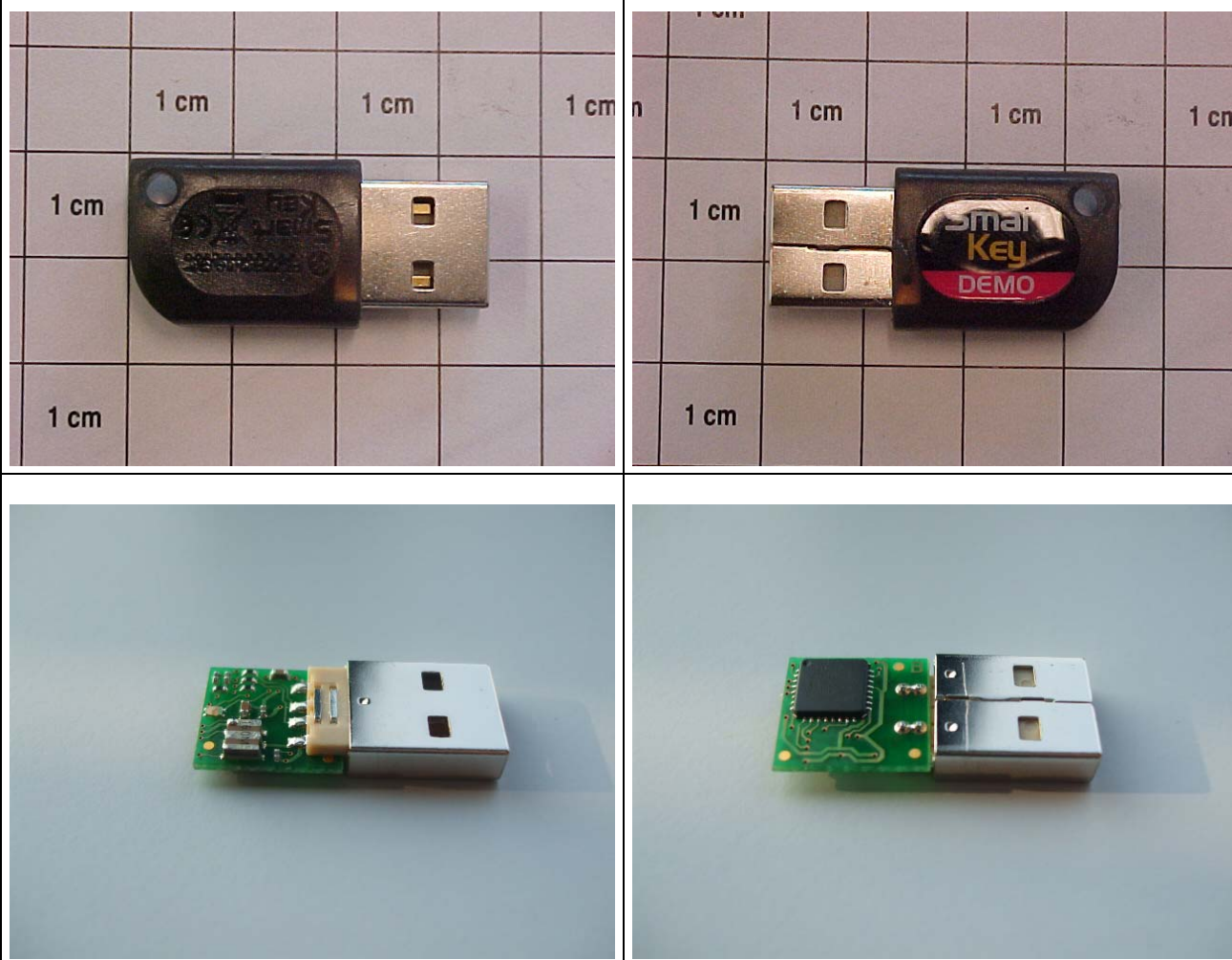
PHOTO No. 1 – EQUIPMENT UNDER TEST
