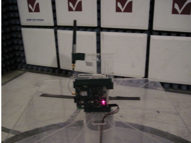
Radio module shown on host board with dipole antenna
