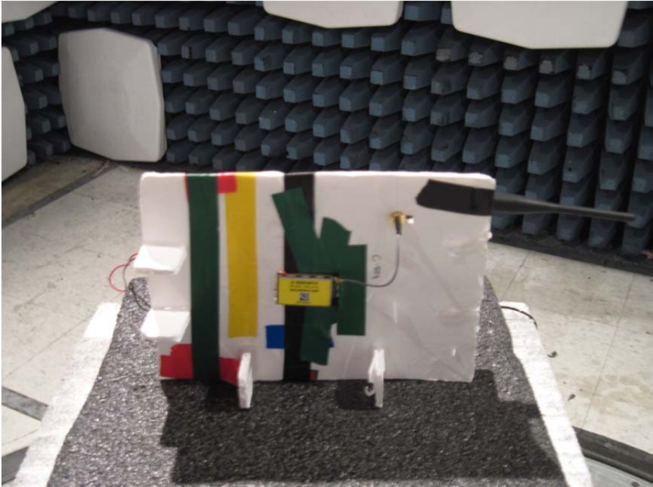
LSR Antenna - Side
