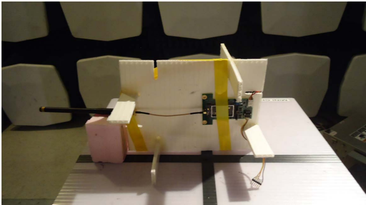
Antenna Factor Antenna - Side
