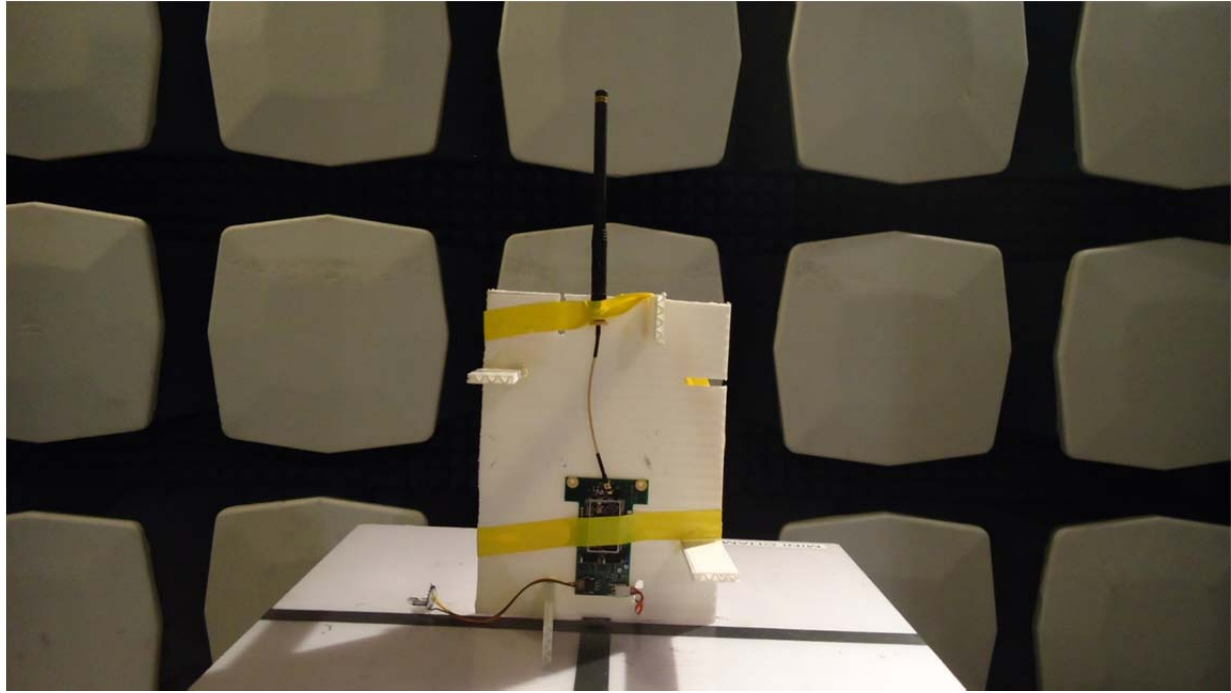
Antenna Factor Antenna - Vertical
