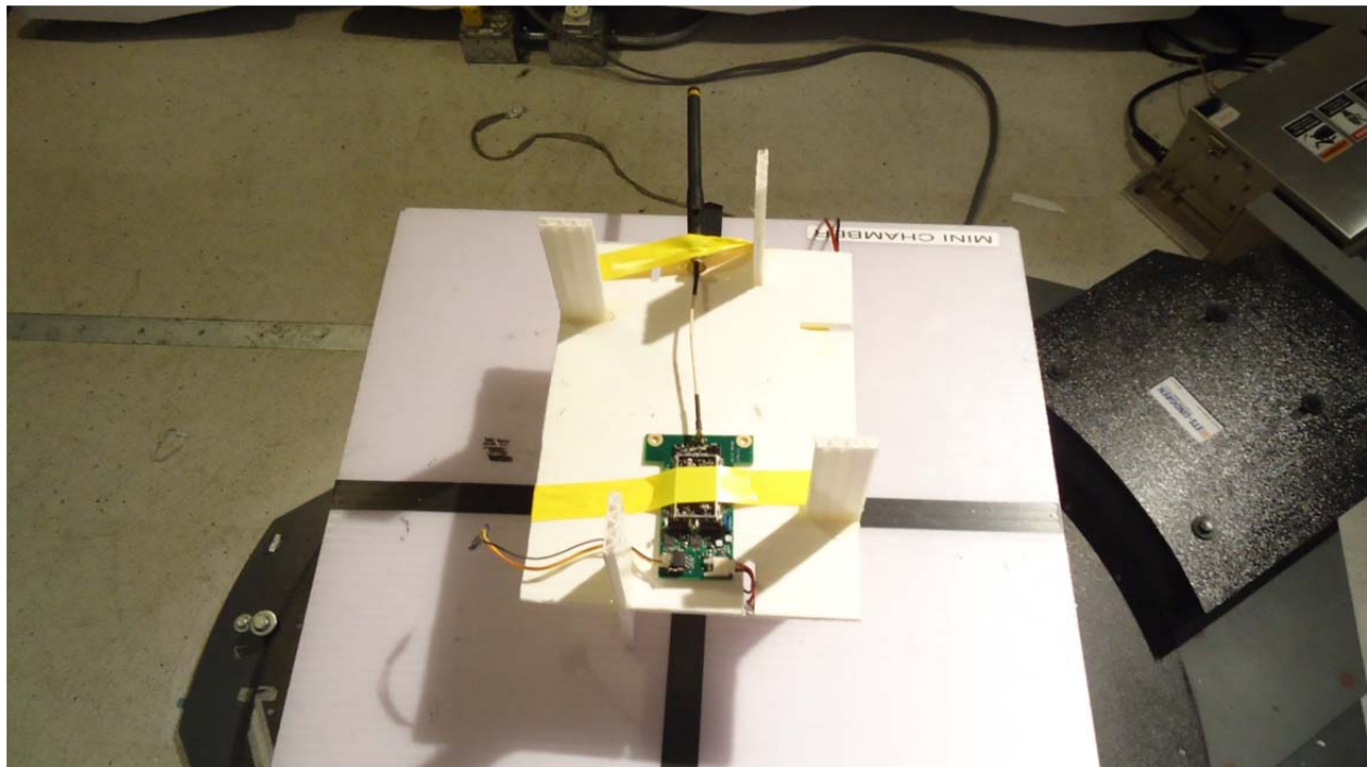
Antenna Factor Antenna - Horizontal
