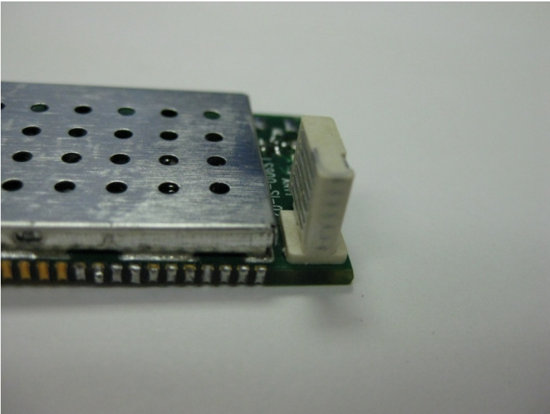
Close Up View #3 of Chip Antenna
