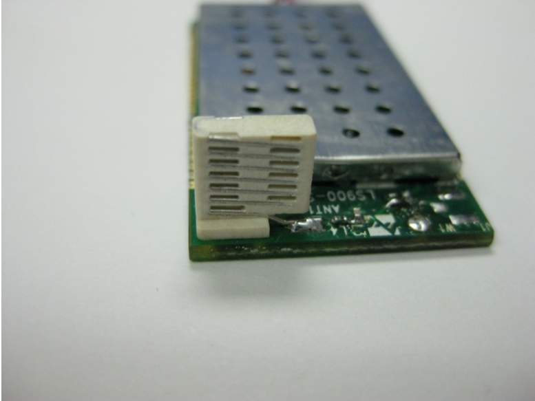
Close Up View #2 of Chip Antenna
