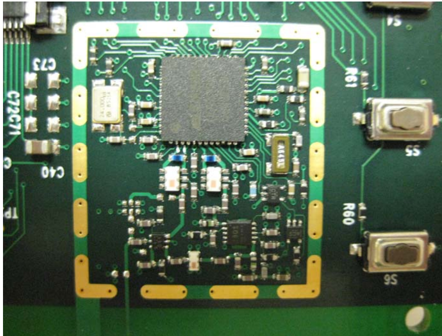
Close Up of RF Section
