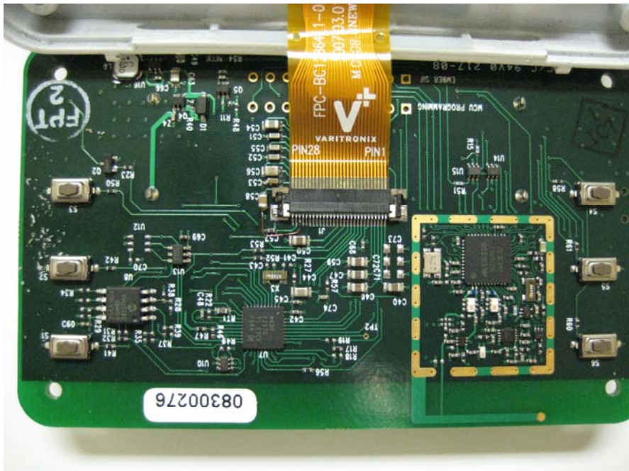
Close Up of Board/RF Section – Shield Removed
