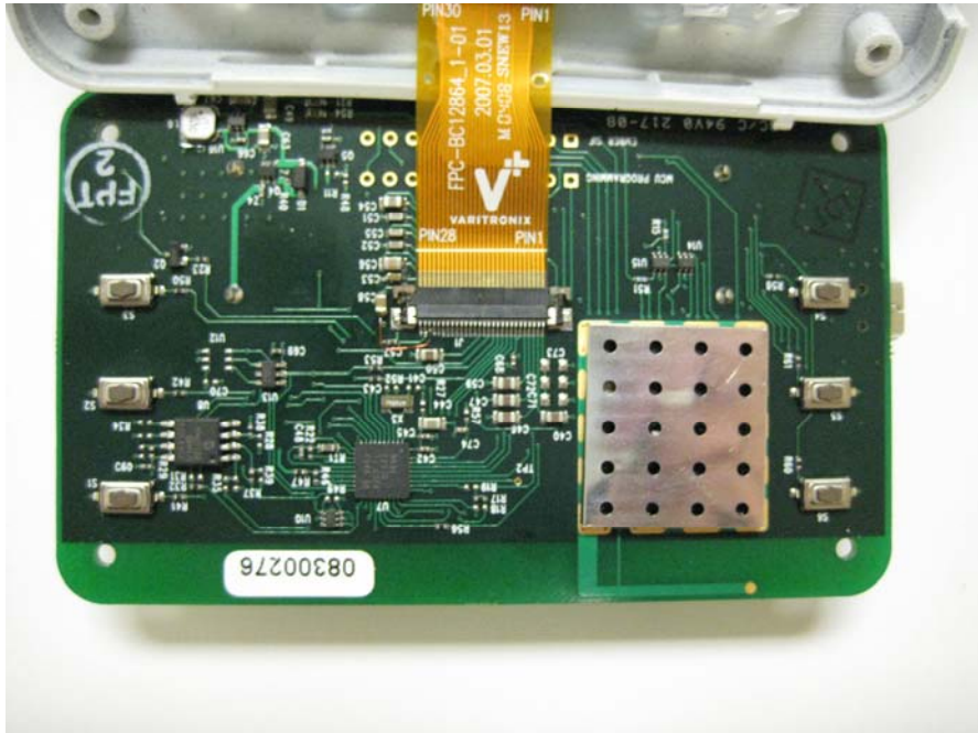
Close Up of Board-RF Section Shielded View #2
