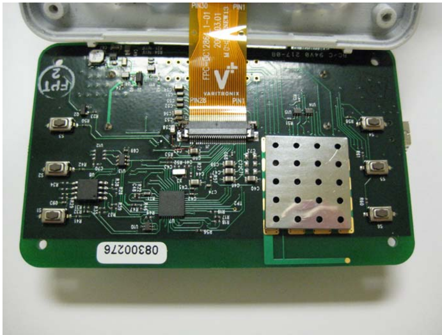
Close Up of Board-RF Section Shielded View #1
