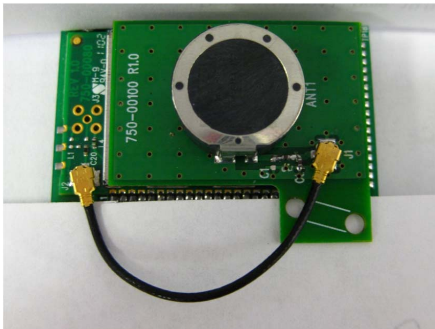
Front side of Board with antenna attached
