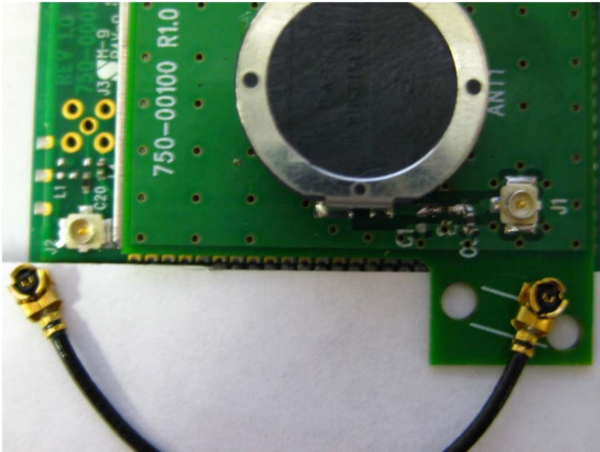
Antenna Connections
