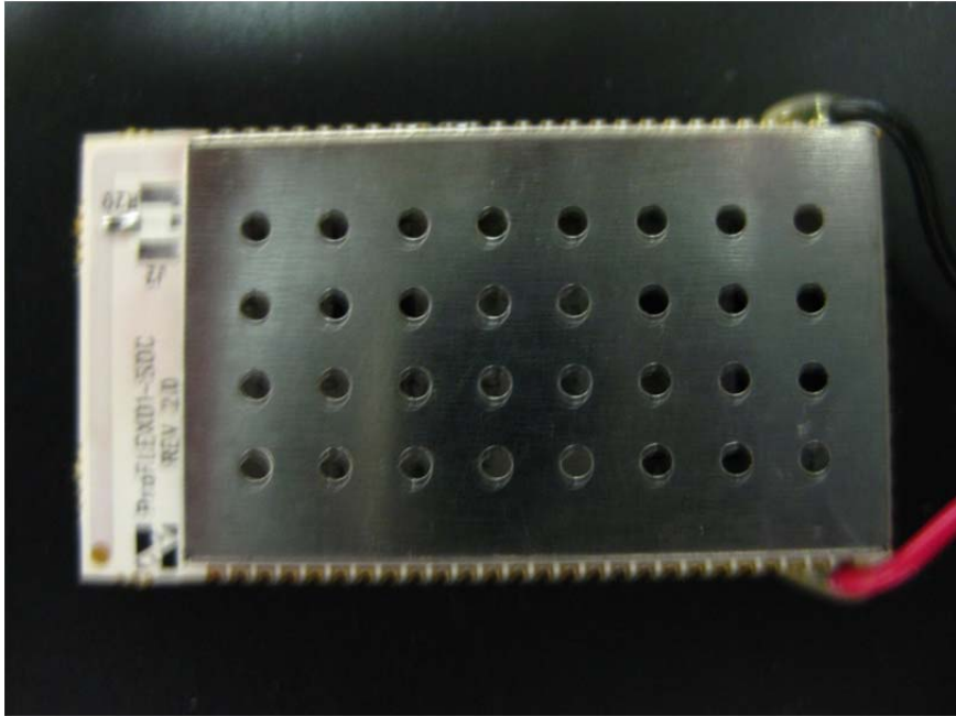
Front side of board with PIFA
