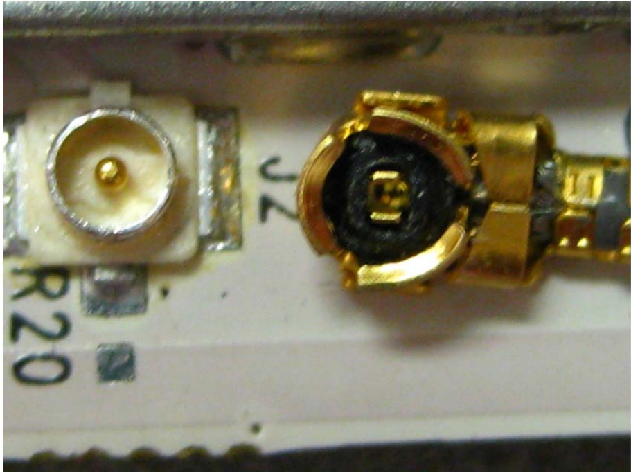
Cable to board connection
