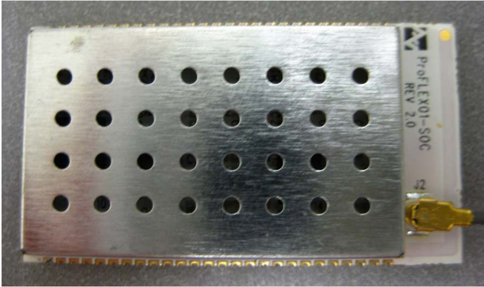
Front side of module with dipole antenna connection
