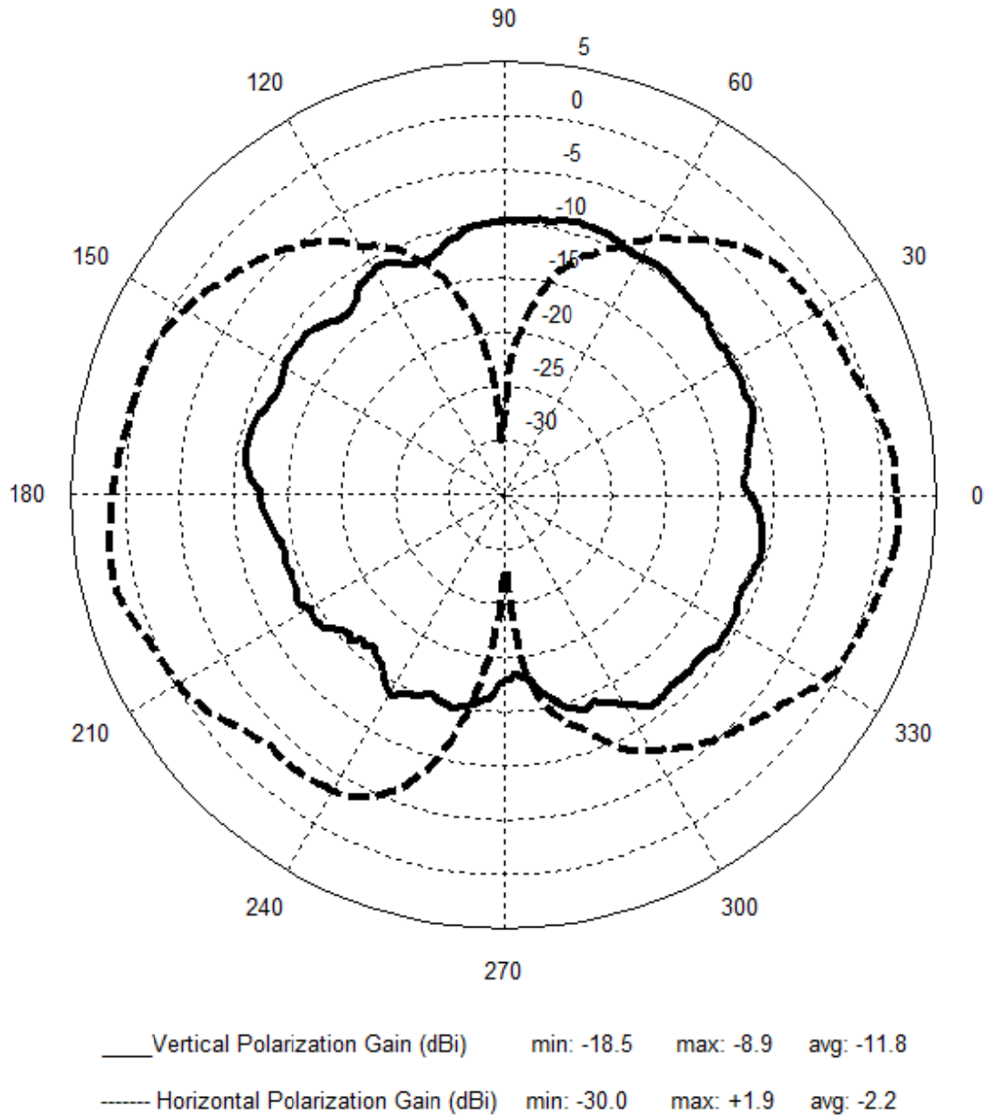
Figure 8 Antenna Power Gain Performance at 2480 MHz, Elevation Pattern
