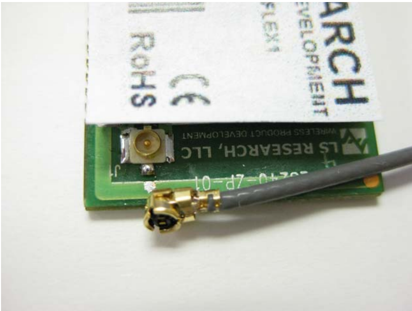
Close up of External Antenna Connection View #1
