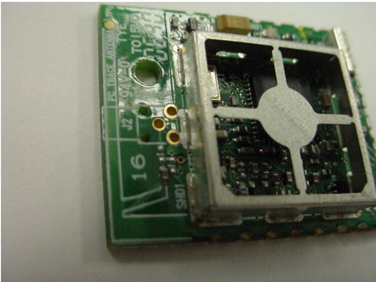
Photo Six – Internal Close Up of PCB Antenna
