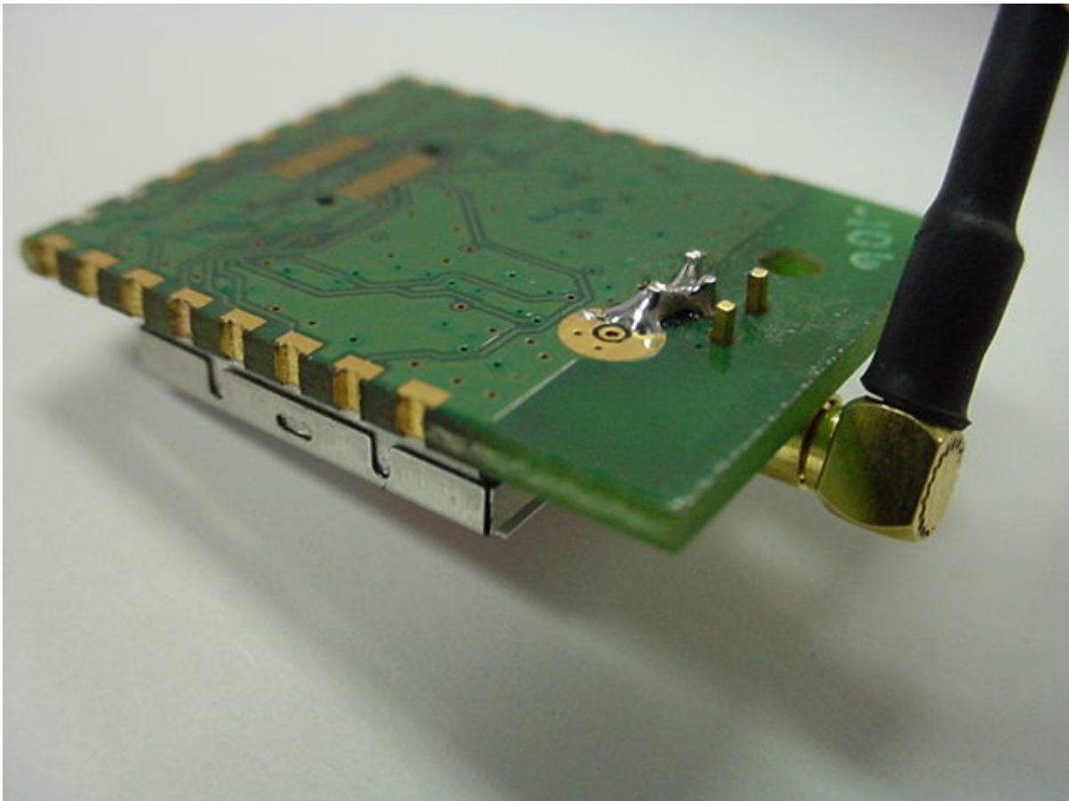
Photo Three – Internal Whip Antenna Connection – Close Up
