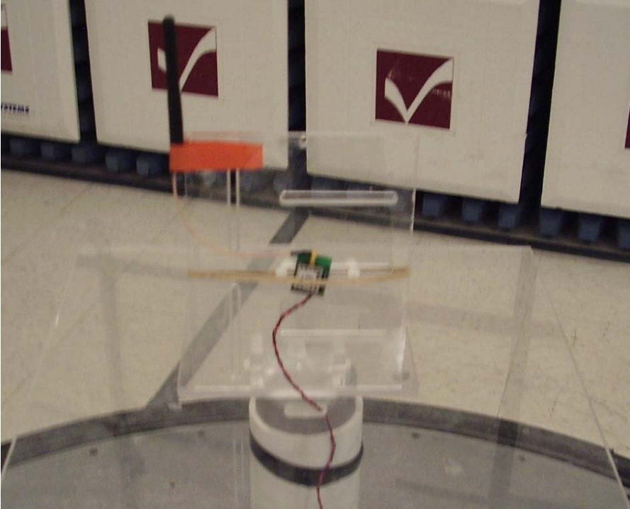
Vertical Orientation, EUT on test pedestal, whip antenna
