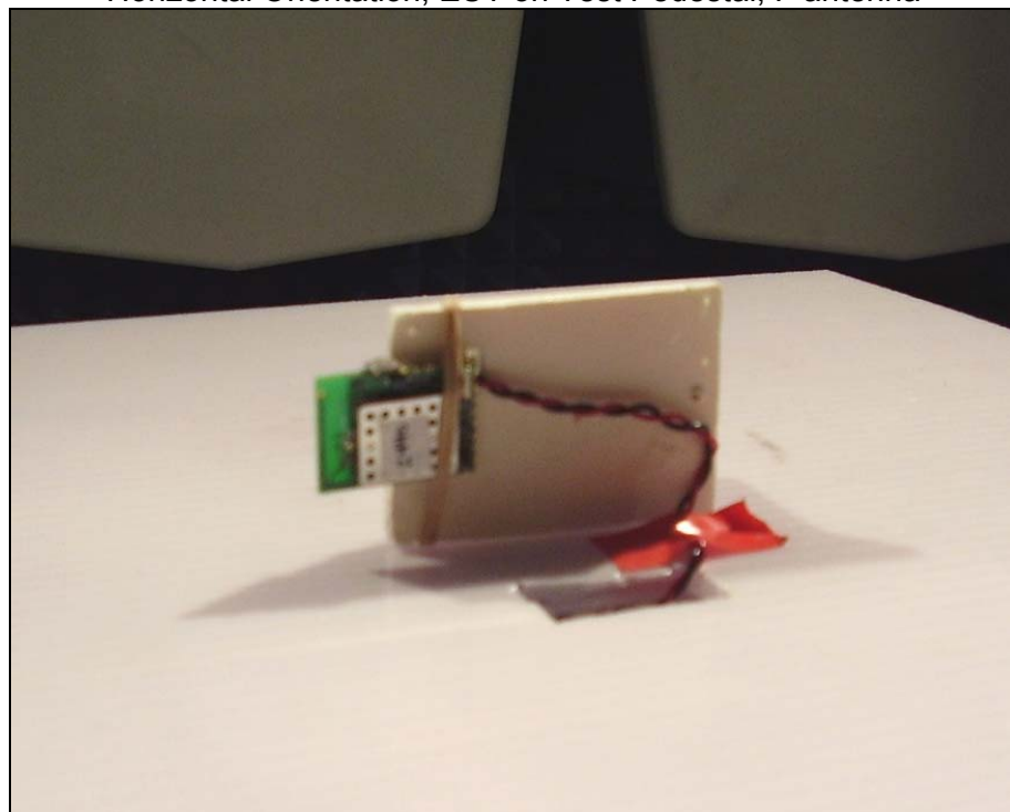
Horizontal Orientation, EUT on Test Pedestal, F antenna
