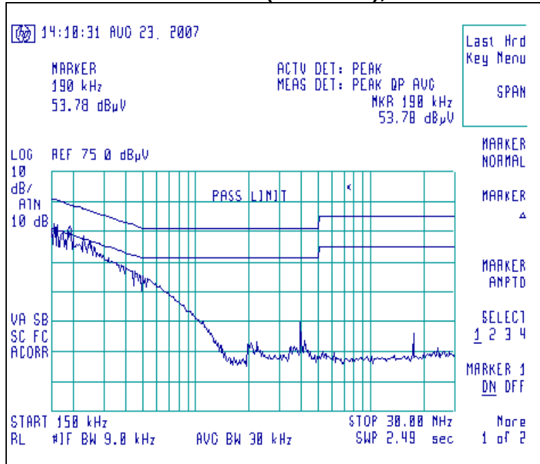
Center Channel (2440 MHz), Line 1
