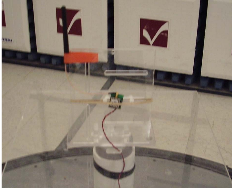
Horizontal Orientation, EUT on test pedestal, whip antenna
