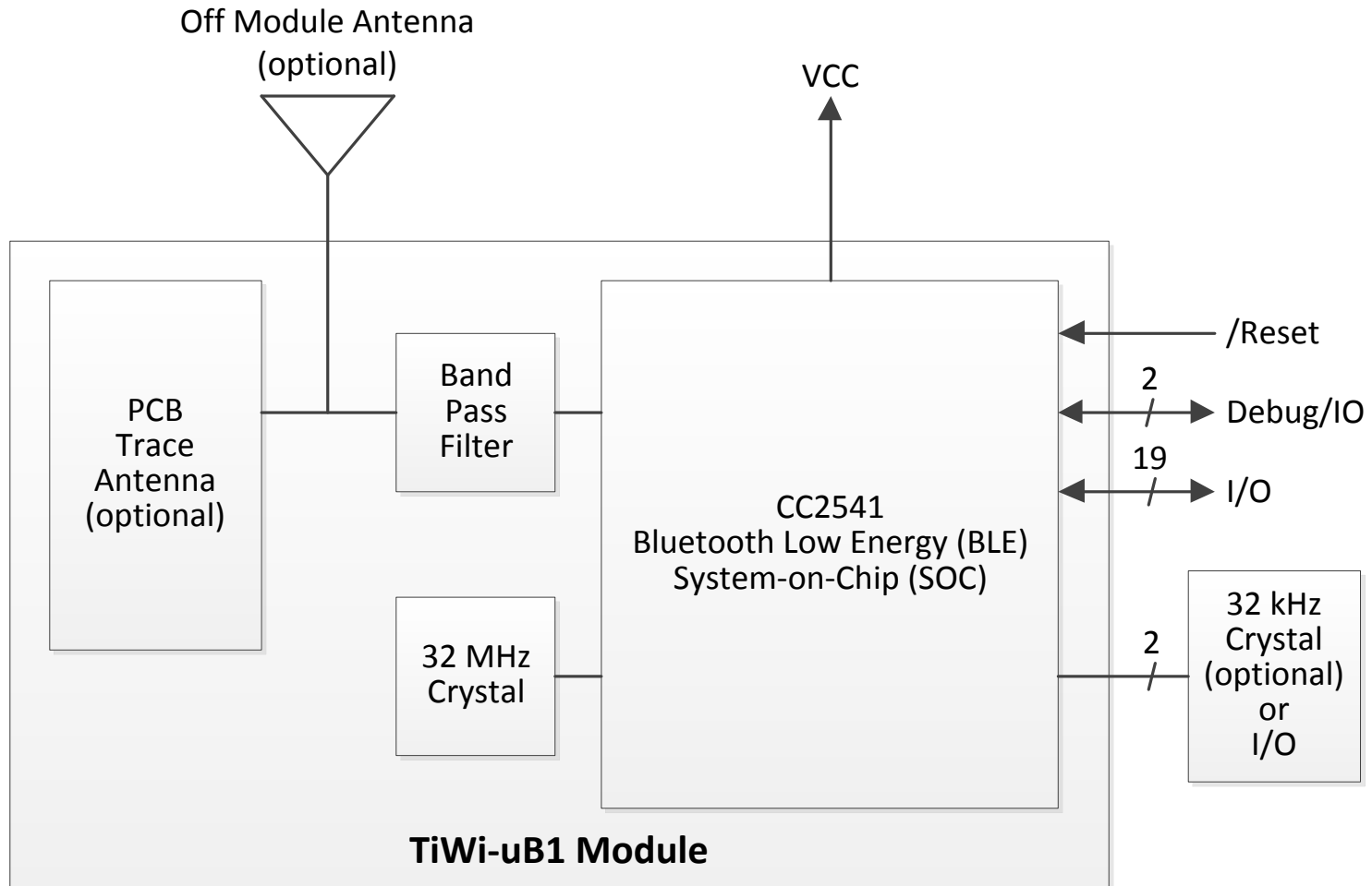
TiWi-uB1 Block Diagram
