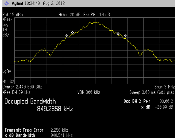
Channel middle -20 dBc Occupied Bandwidth
