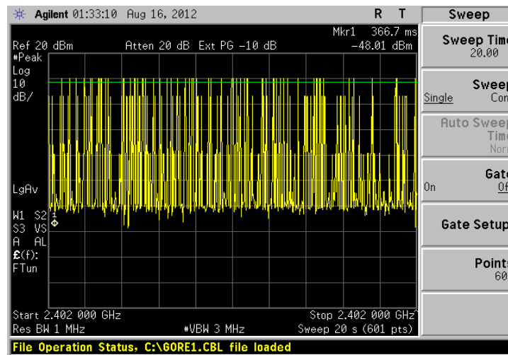
A 20 sec screen captures shows 52 transmissions
