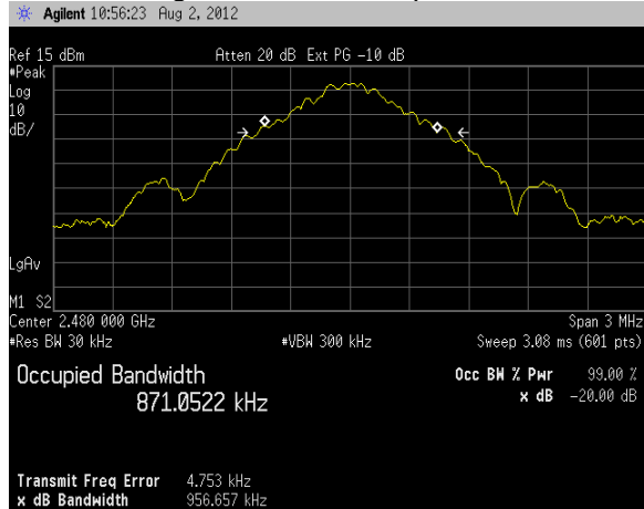
Channel high -20 dBc Occupied Bandwidth
