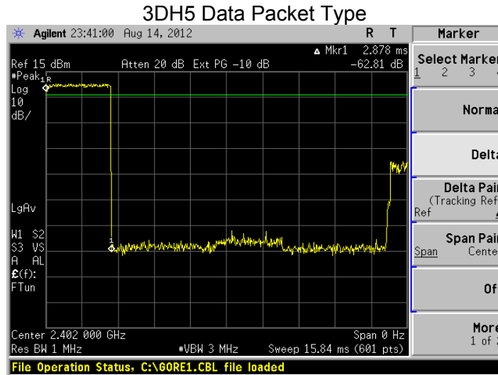
Maximum on-time, 2.878ms, demonstrated with 3DH5 Data Packet Type enabled
