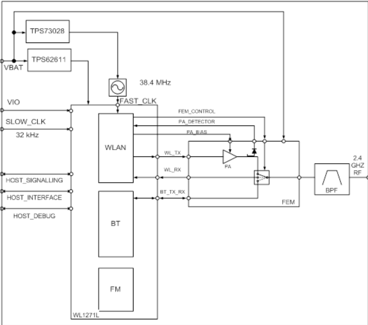
Figure 1 - TiWi-BLECA Block Diagram
