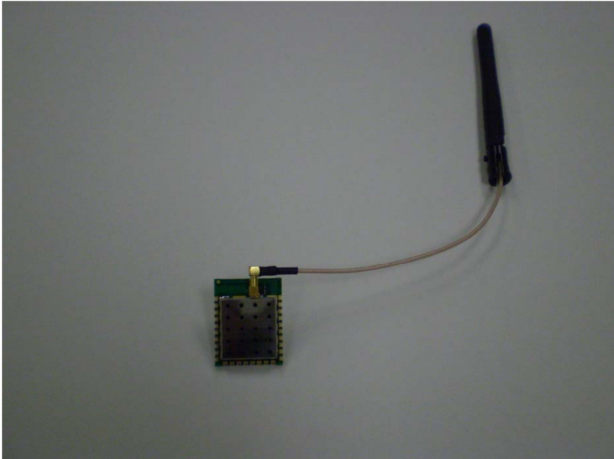
Photo Five – External View of Module, Showing External Nearson Antenna Connected
