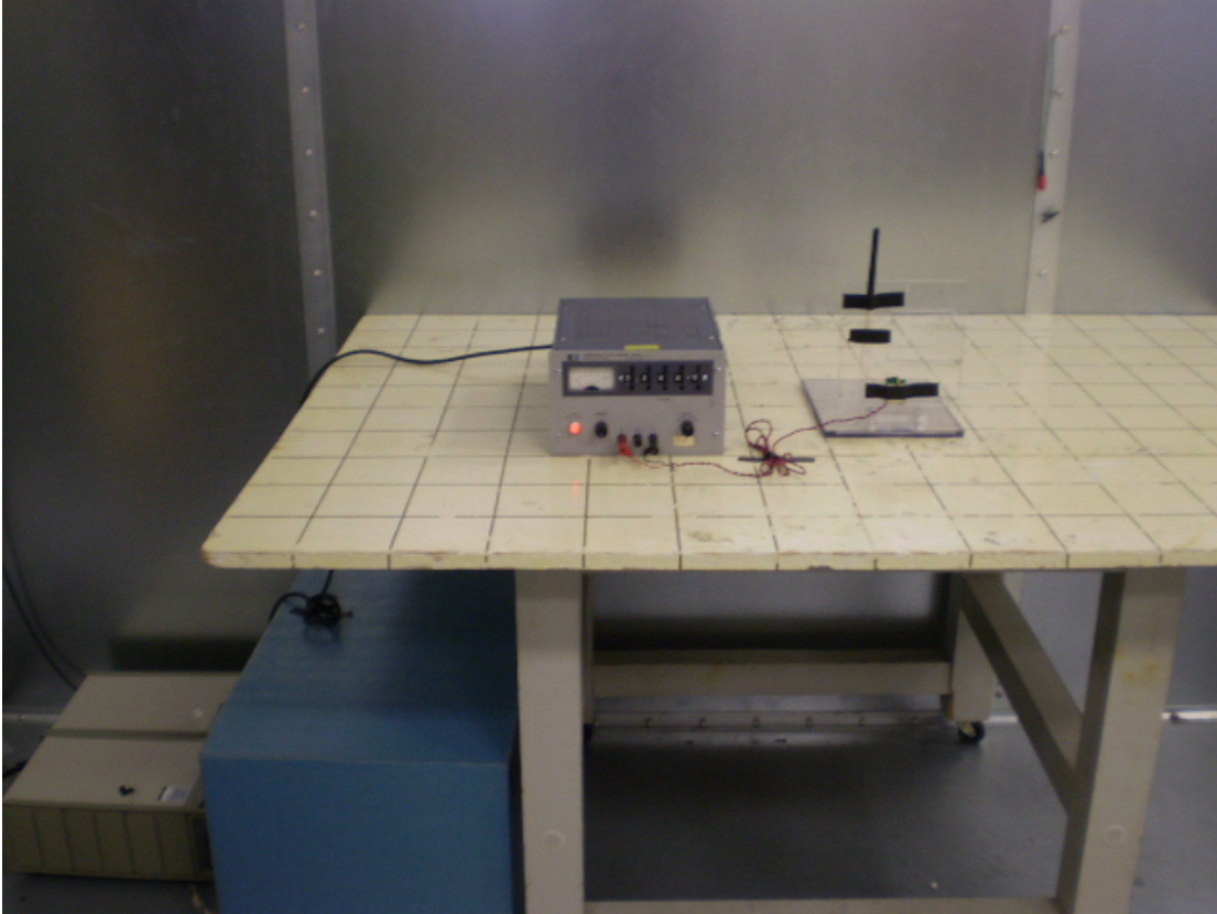
Test Setup Photo(s) – Conducted Emissions Test (with DiPole Antenna)
