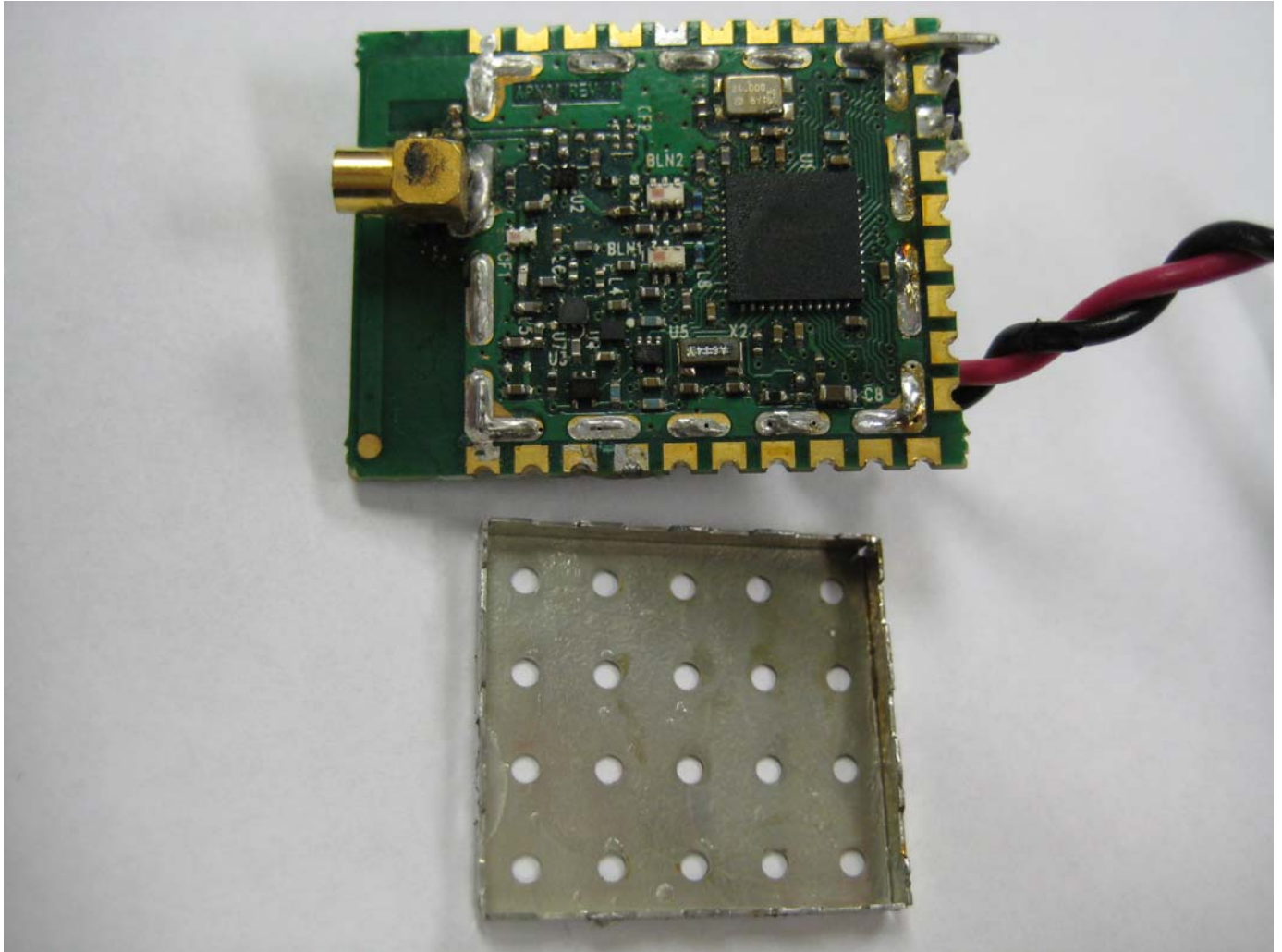
View 2 of Board – Shield Removed (DiPole Antenna)
