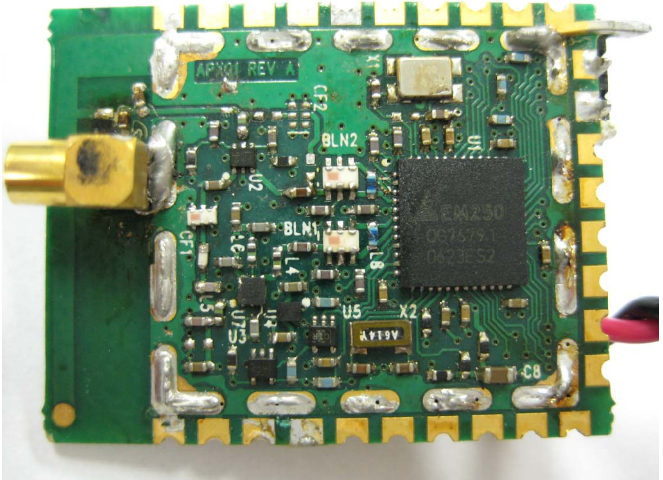
View 1 of Board – Shield Removed (DiPole Antenna)
