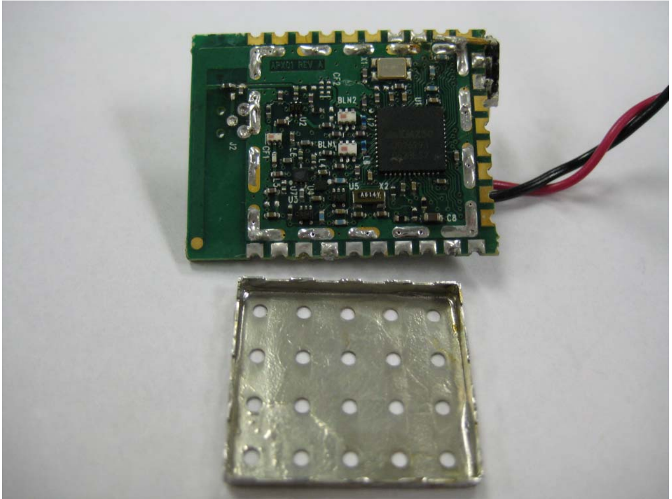
View 2 of Board – Shield Removed (PCB Trace Antenna)
