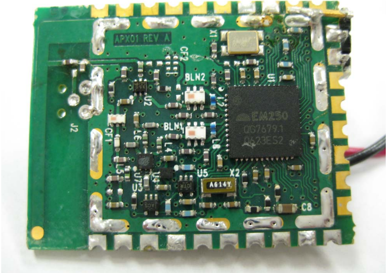
View 1 of Board – Shield Removed (PCB Trace Antenna)
