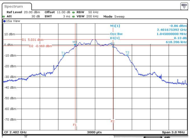
99% Occupied Bandwidth-1Mbps
