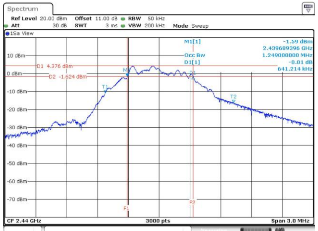
99% Occupied Bandwidth-1Mbps
