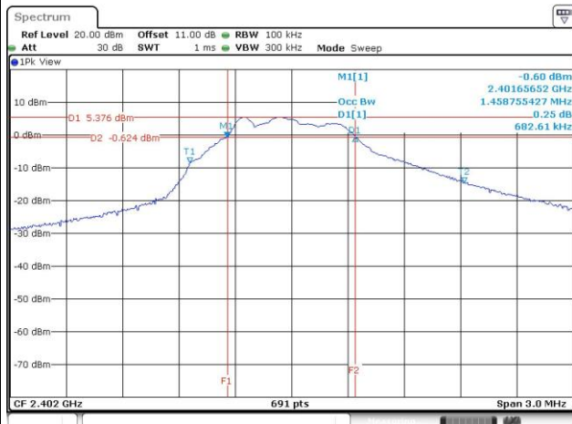
6dB Bandwidth-1Mbps
