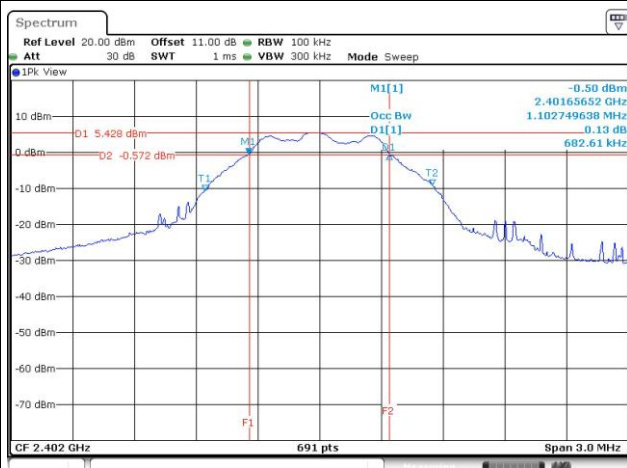
6dB Bandwidth-1Mbps
