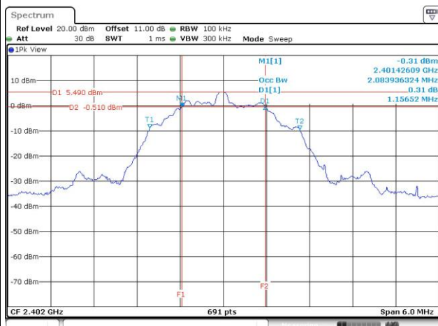
6dB Bandwidth-2Mbps
