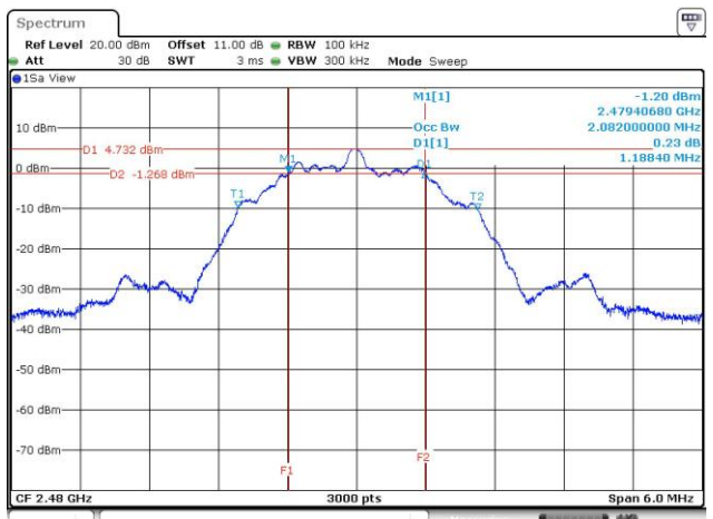
99% Occupied Bandwidth-2Mbps
