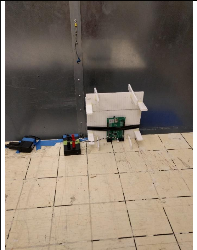
Conducted AC Emissions Setup
