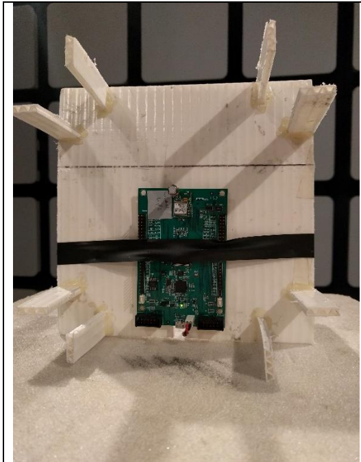
Vertical EUT Orientation
