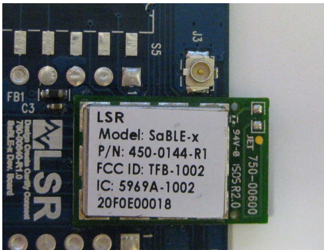
Module with u.fl connector
