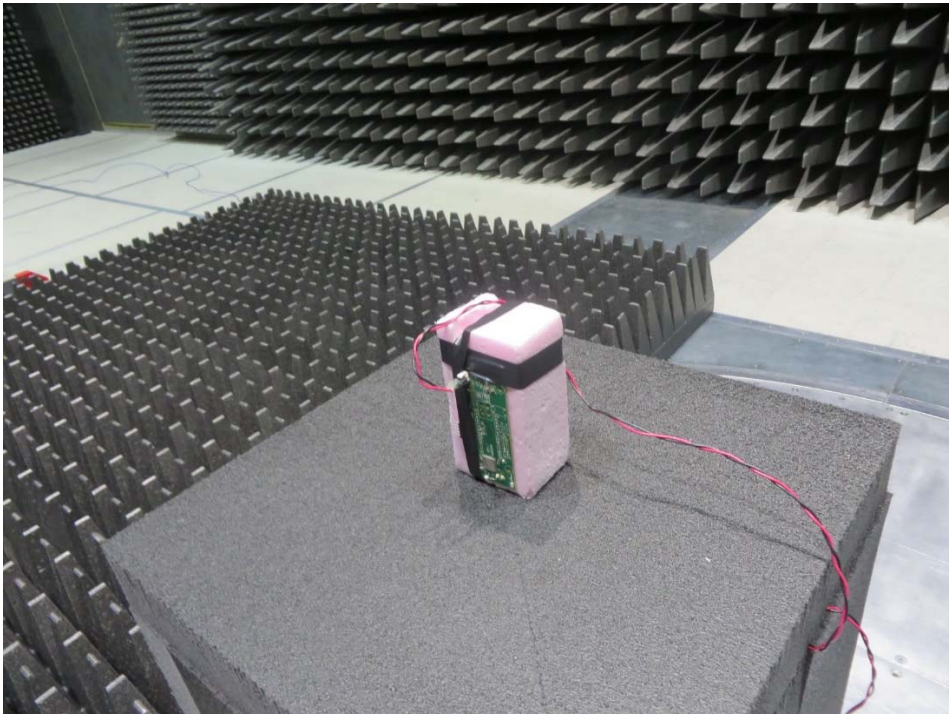
Horizontal – 2-layer Design
