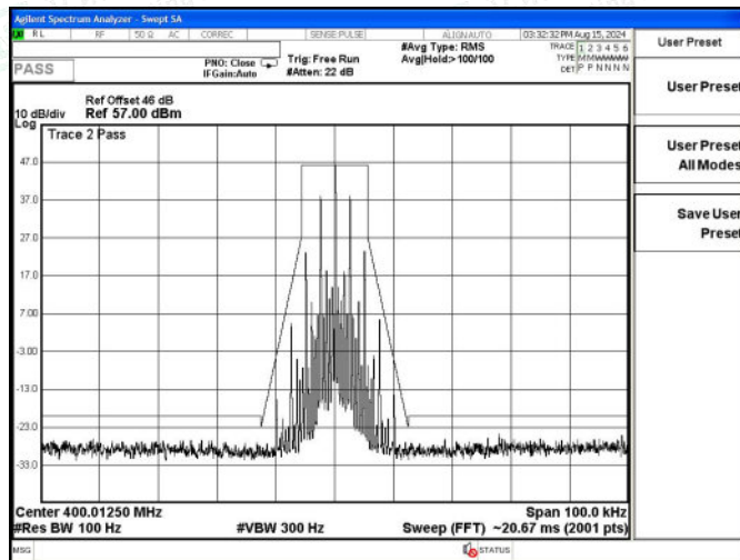
Mask_High Power Level FM 12.5kHz
