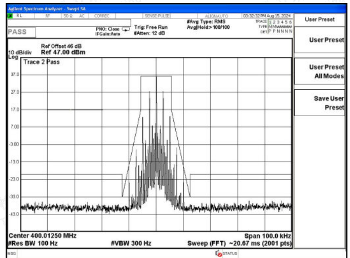
Mask_Low Power Level FM 12.5kHz
