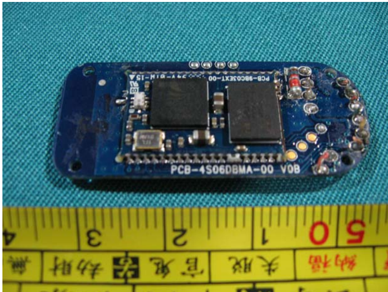
Back view of Main board
