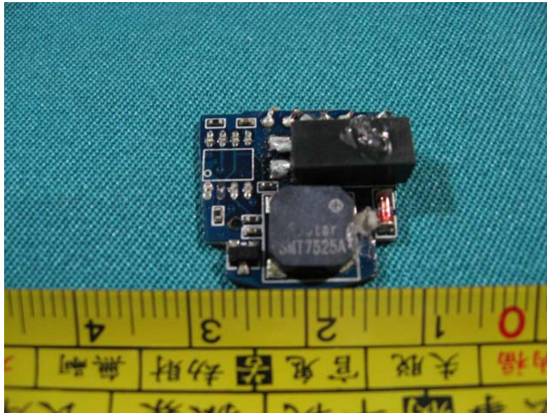
Front View of Daughter board
