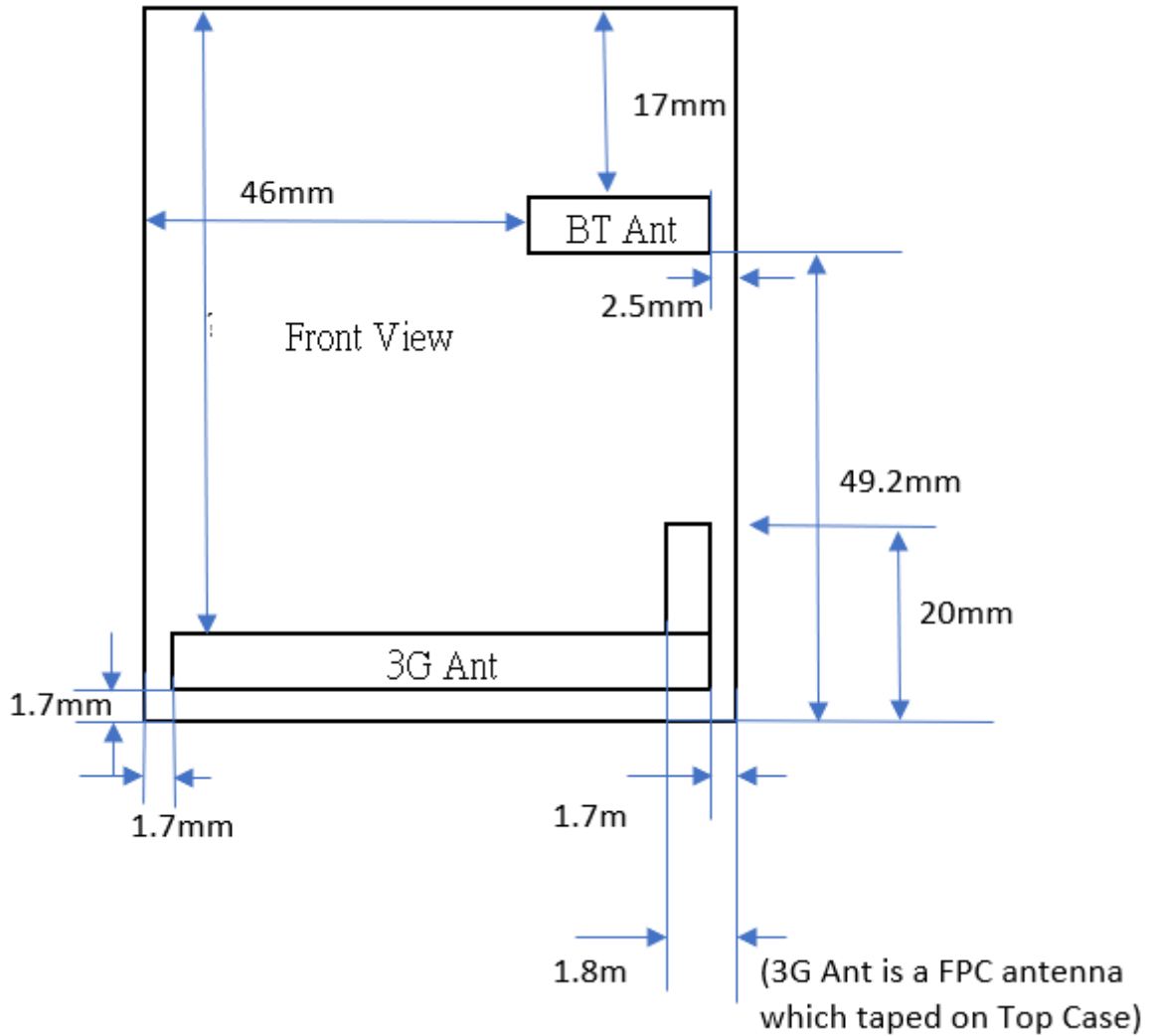
Fig.7 Antenna location
