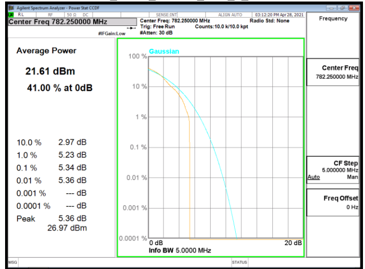
Band13_10MHz_16QAM_RB1_0_CH23230
