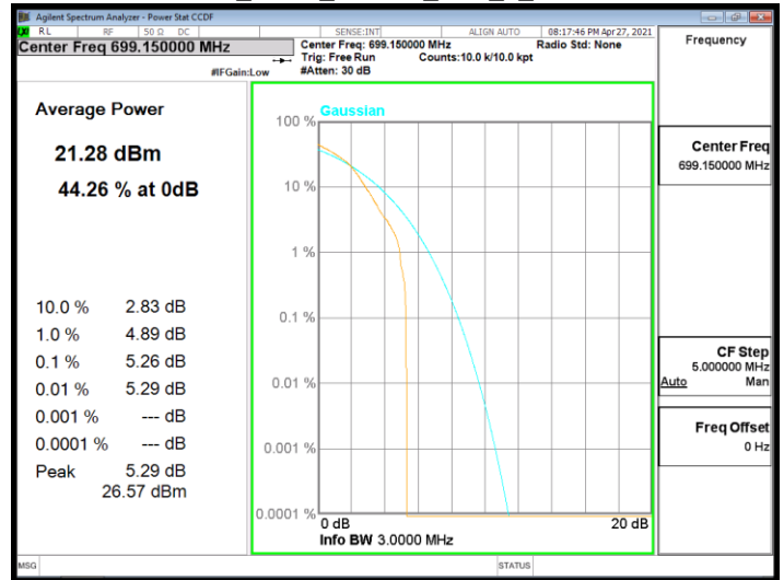
Band12_3MHz_16QAM_RB1_0_CH23095
