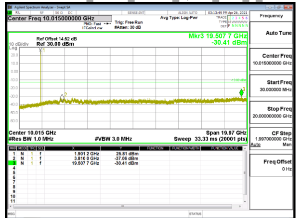
Spurious Emission_Band2_10MHz_QPSK_RB1_0_CH19150
