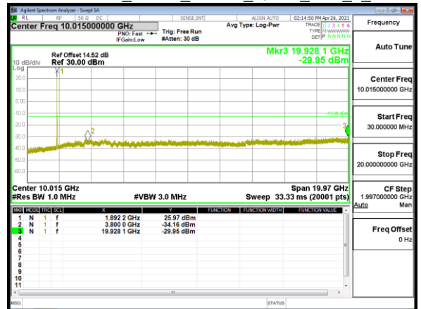
Spurious Emission_Band2_20MHz_QPSK_RB1_0_CH19100
