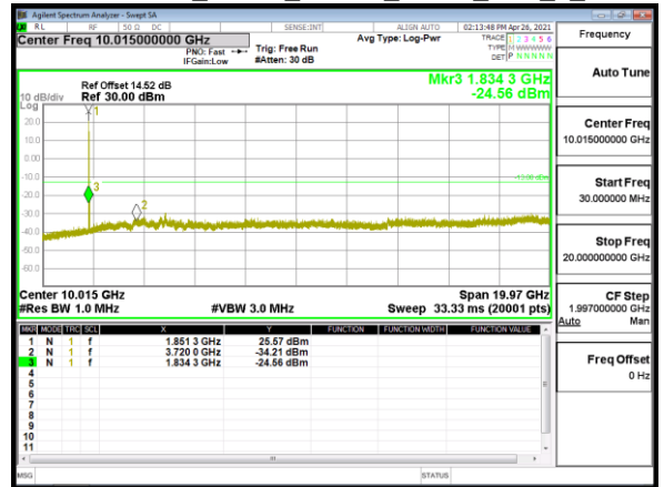
Spurious Emission_Band2_20MHz_QPSK_RB1_0_CH18900
