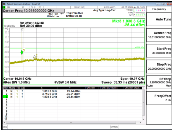
Spurious Emission_Band2_15MHz_QPSK_RB1_0_CH18900
