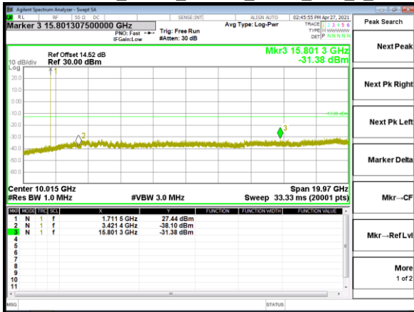
Spurious Emission_Band4_1.4MHz_QPSK_RB1_0_CH20175
