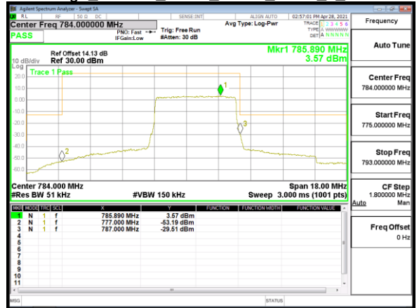
Band Edge_Band13_5MHz_QPSK_RB25_0_CH23255
