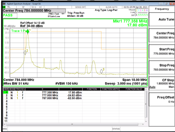
Band Edge_Band13_5MHz_QPSK_RB1_0_CH23205
