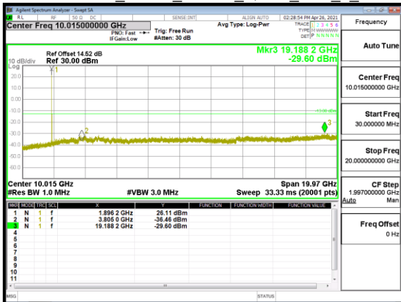
Spurious Emission_Band2_15MHz_QPSK_RB1_0_CH19125
