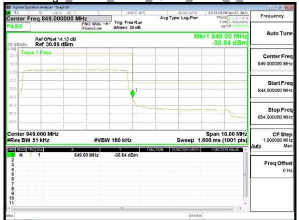
Band Edge_Band5_5MHz_QPSK_RB25_0_CH20625
