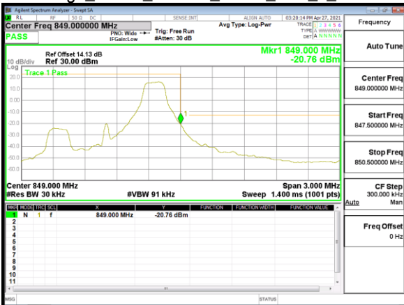
Band Edge_Band5_1.4MHz_QPSK_RB6_0_CH20407
