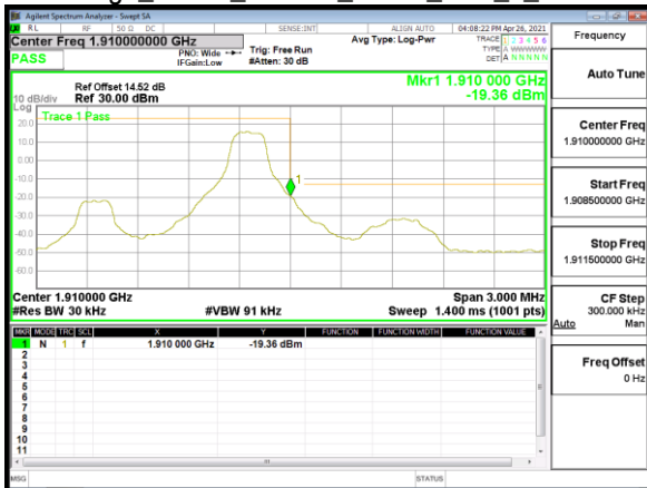
Band Edge_Band2_1.4MHz_QPSK_RB6_0_CH18607
