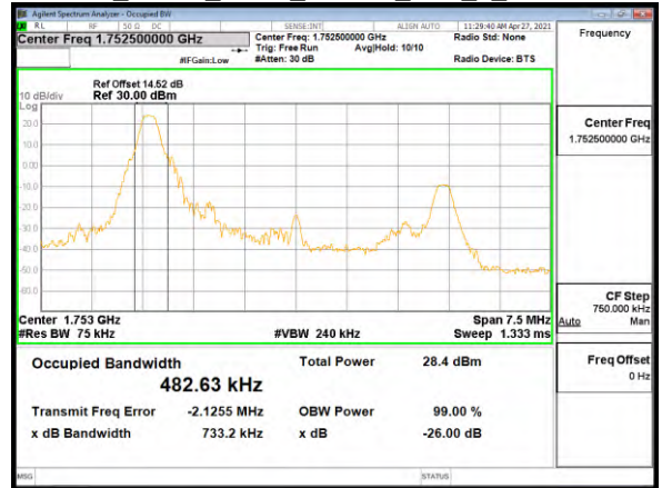
OBW_Band4_5MHz_16QAM_RB1_0_CH20375
