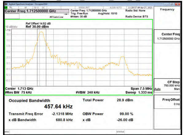
OBW_Band4_5MHz_16QAM_RB1_0_CH20175
