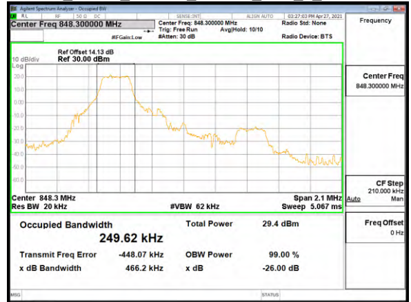
OBW_Band5_1.4MHz_16QAM_RB1_0_CH20643
