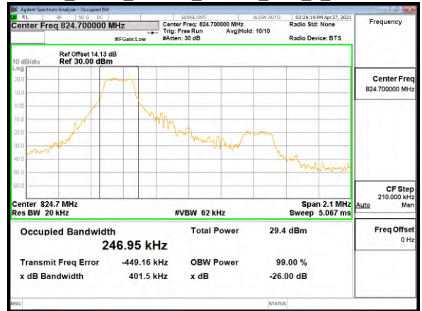
OBW_Band5_1.4MHz_16QAM_RB1_0_CH20525
