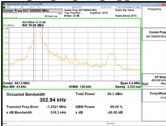
OBW_Band5_3MHz_16QAM_RB1_0_CH20635
