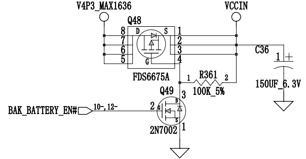
MAX1636 OUTPUT
