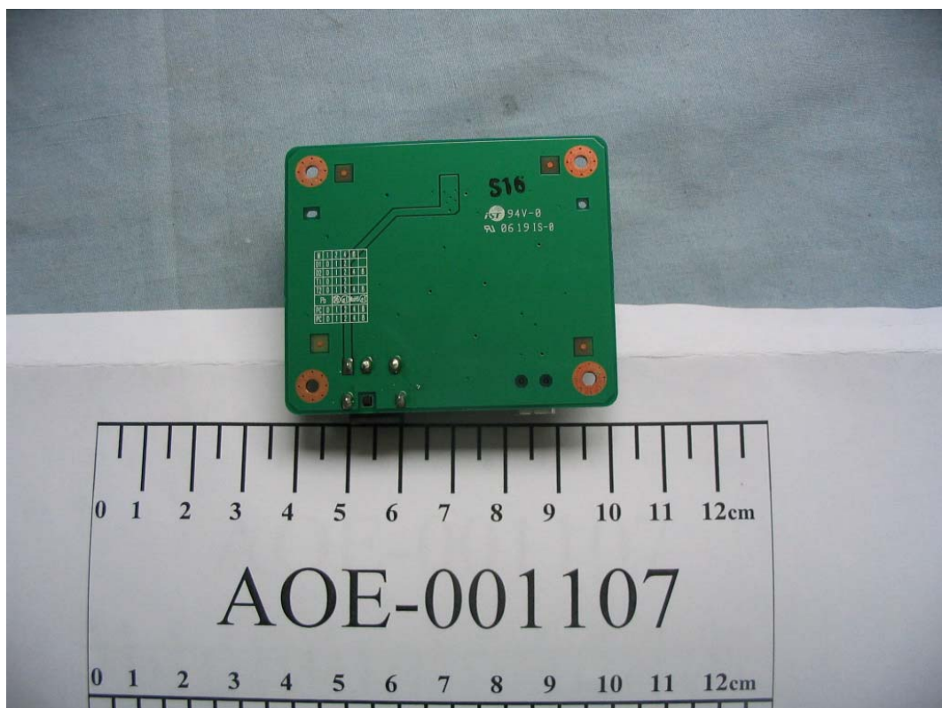
FIGURE 31 WIRELESS POINT OF SALE PDA (M/N: MRT320) CHARGING CRADLE BOARD 1 (SIDE 1)
