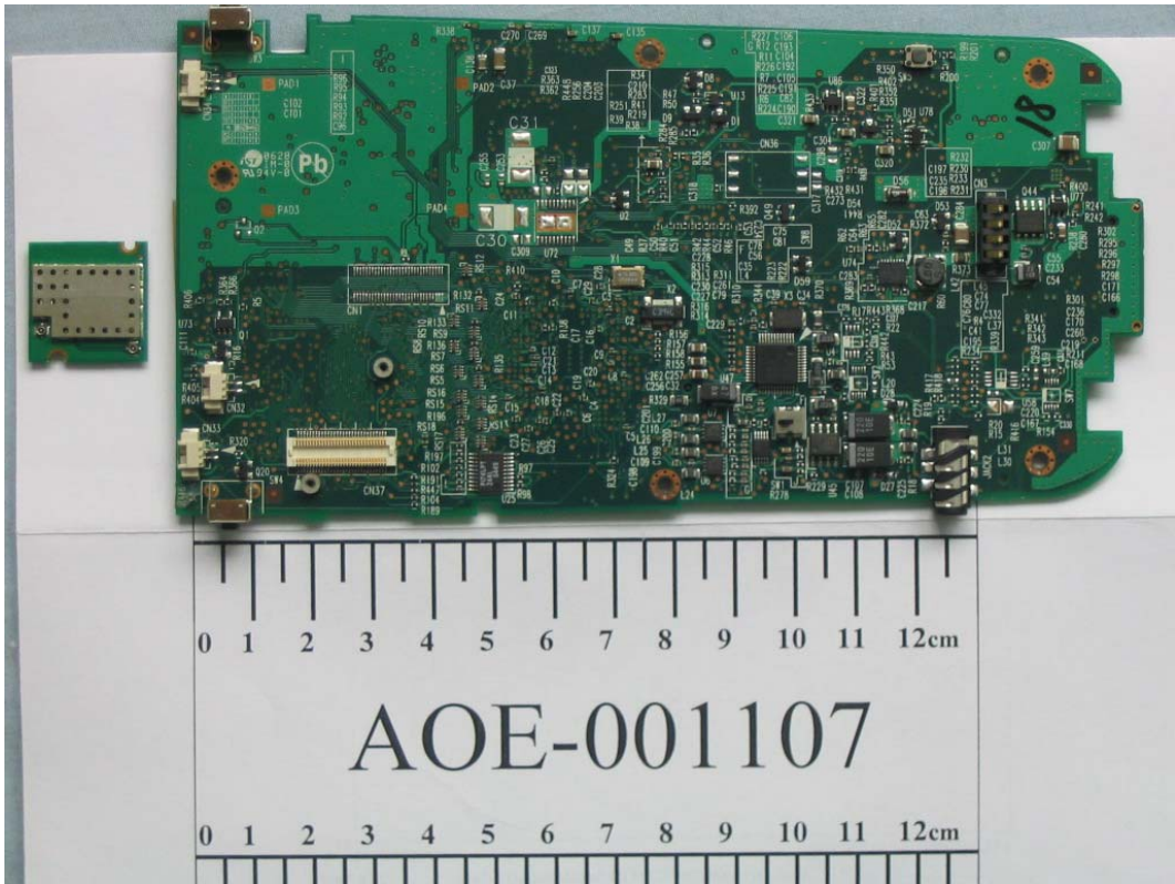
FIGURE 5 WIRELESS POINT OF SALE PDA (M/N: MRT320) HAND-HELD UNIT MAIN BOARD (RF MODULE REMOVED)
