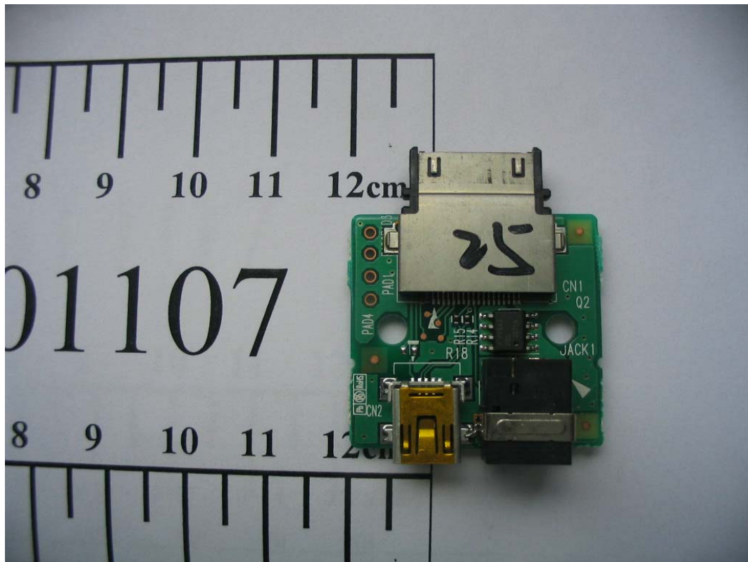
FIGURE 26 WIRELESS POINT OF SALE PDA (M/N: MRT320) MINI ADAPTOR MAIN BOARD (COMPONENT VIEW)
