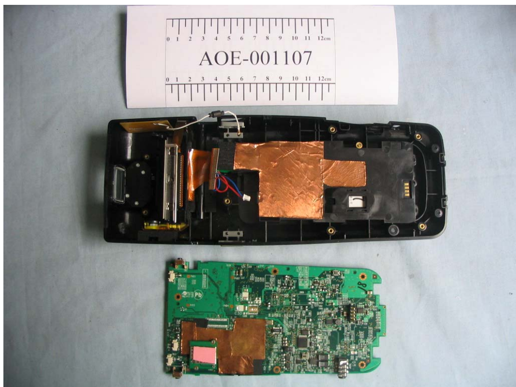
FIGURE 2 WIRELESS POINT OF SALE PDA (M/N: MRT320) HAND-HELD UNIT COVER REMOVED 2
