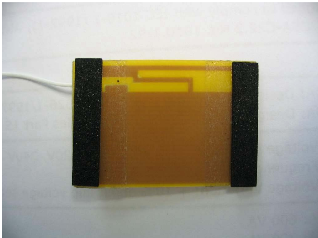
FIGURE 14 WIRELESS POINT OF SALE PDA (M/N: MRT320) ANTENNA (BACK VIEW)
