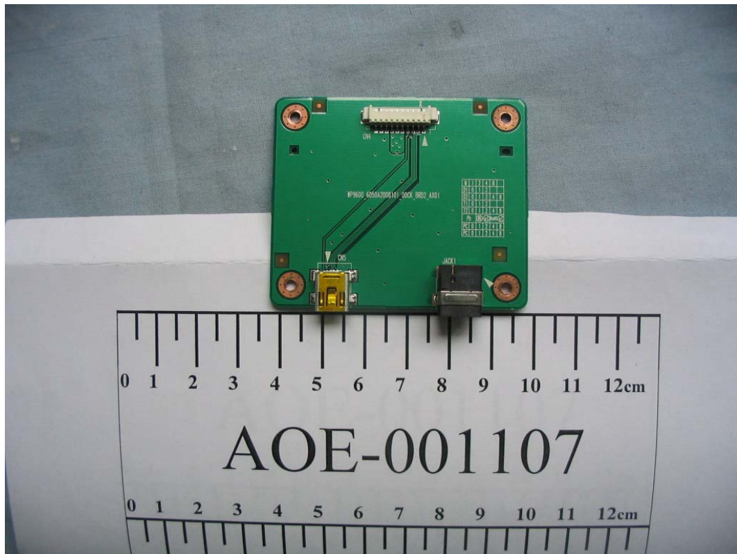
FIGURE 32 WIRELESS POINT OF SALE PDA (M/N: MRT320) CHARGING CRADLE BOARD 1 (SIDE 2)
