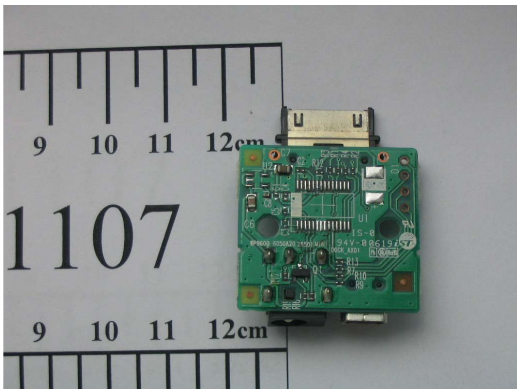
FIGURE 27 WIRELESS POINT OF SALE PDA (M/N: MRT320) MINI ADAPTOR MAIN BOARD (SOLDERED VIEW)
