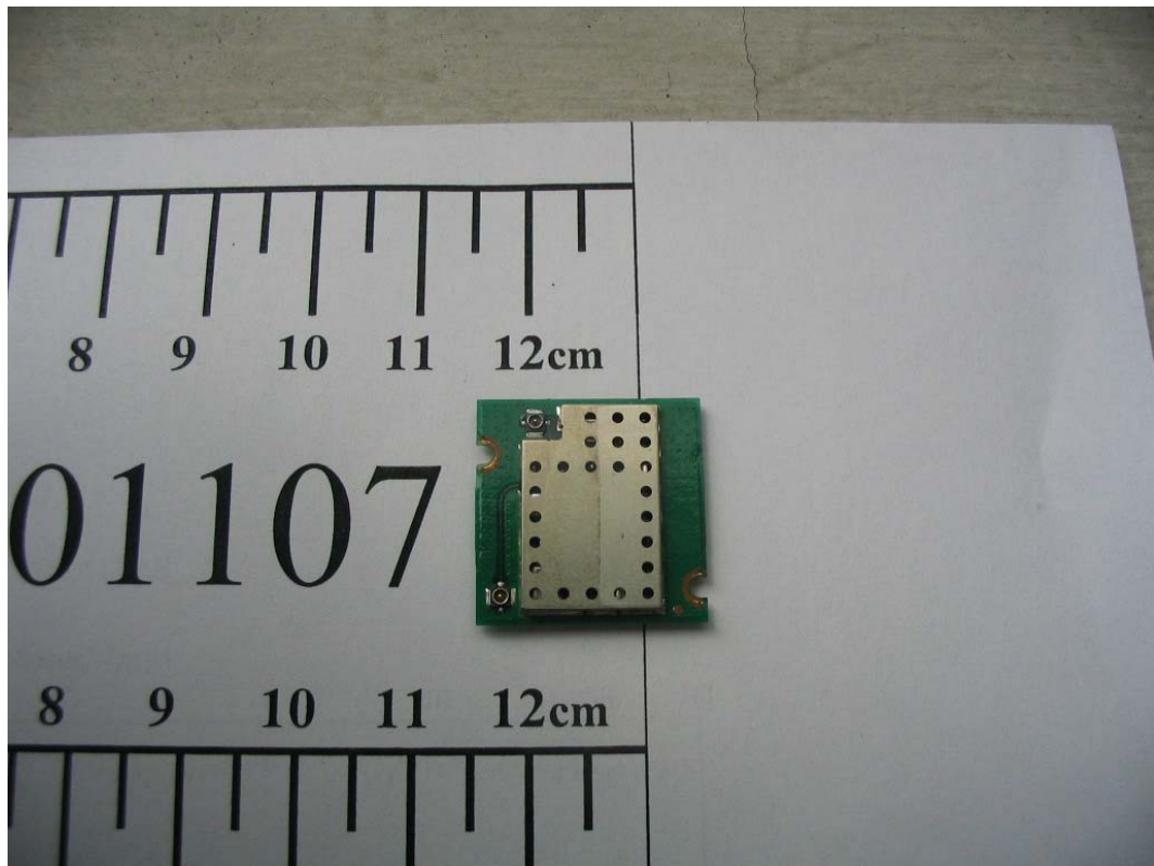
FIGURE 9 WIRELESS POINT OF SALE PDA (M/N: MRT320) HAND-HELD UNIT RF MODULE (SIDE 1)
