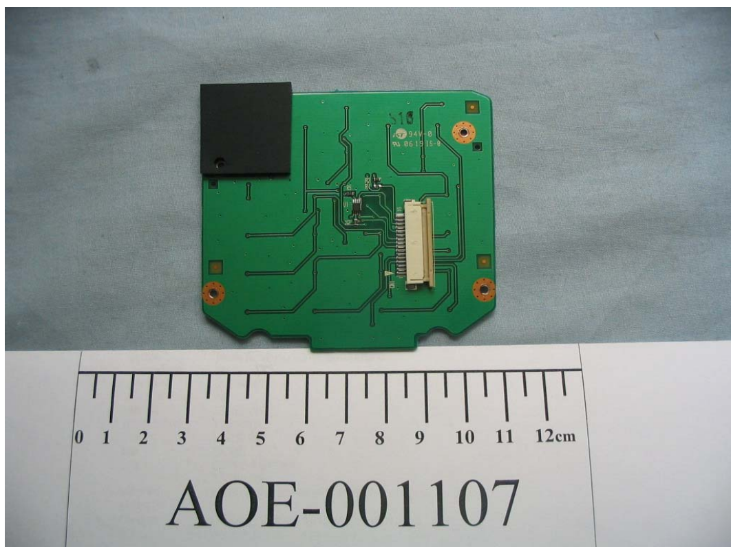
FIGURE 17 WIRELESS POINT OF SALE PDA (M/N: MRT320) HAND-HELD UNIT BUTTON BOARD (SIDE 1)
