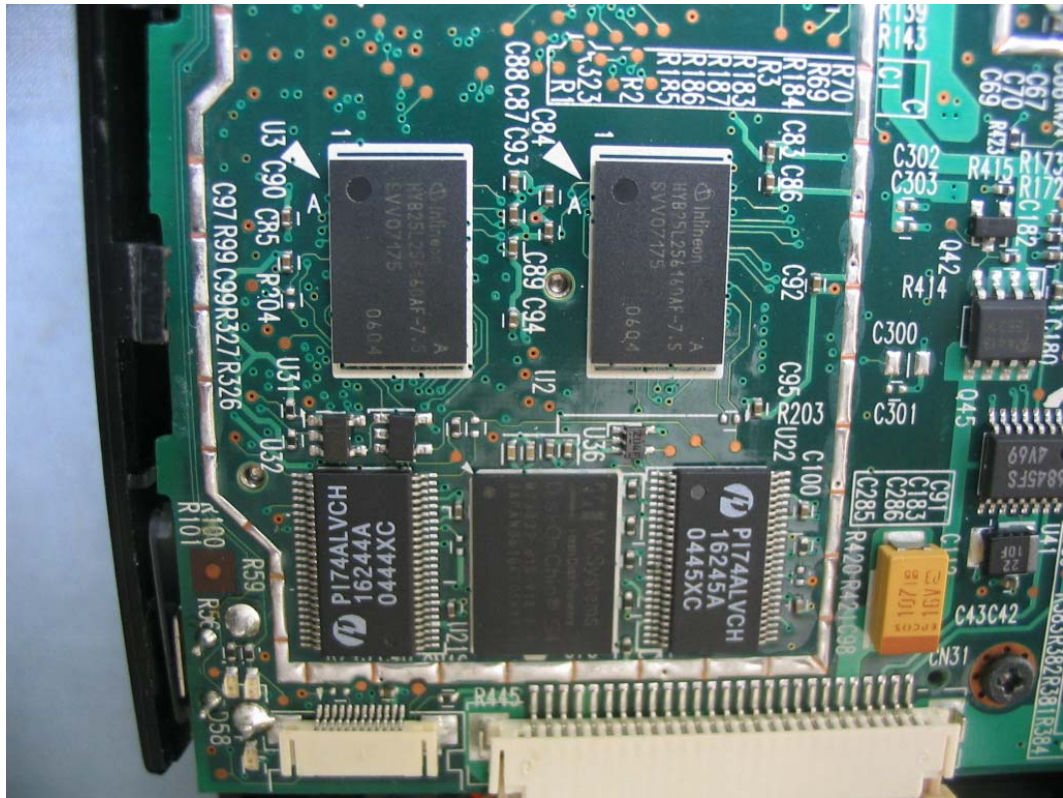
FIGURE 7 WIRELESS POINT OF SALE PDA (M/N: MRT320) CHIPS ON MAIN BOARD 2
