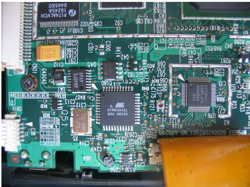
FIGURE 8 WIRELESS POINT OF SALE PDA (M/N: MRT320) CHIPS & CRYSTAL ON MAIN BOARD 3
