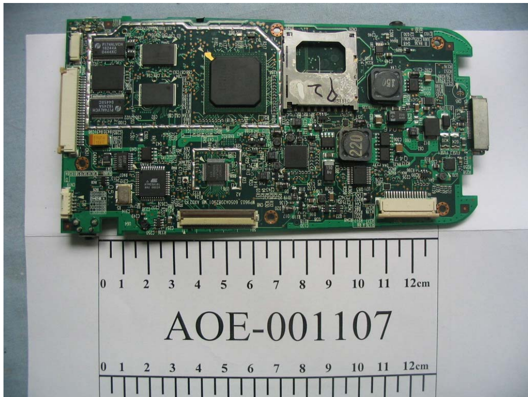
FIGURE 3 WIRELESS POINT OF SALE PDA (M/N: MRT320) HAND-HELD UNIT MAIN BOARD (COMPONENT SIDE)
