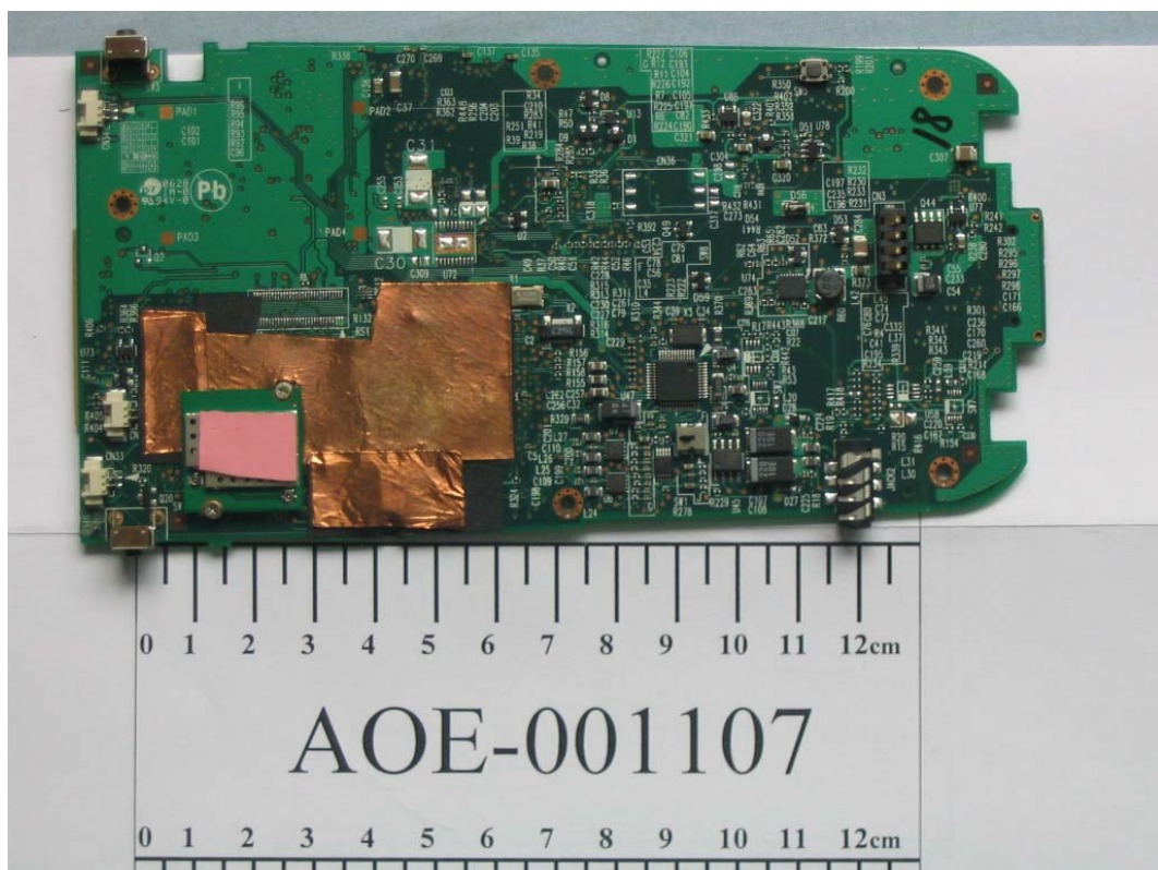
FIGURE 4 WIRELESS POINT OF SALE PDA (M/N: MRT320) HAND-HELD UNIT MAIN BOARD (SOLDERED SIDE)
