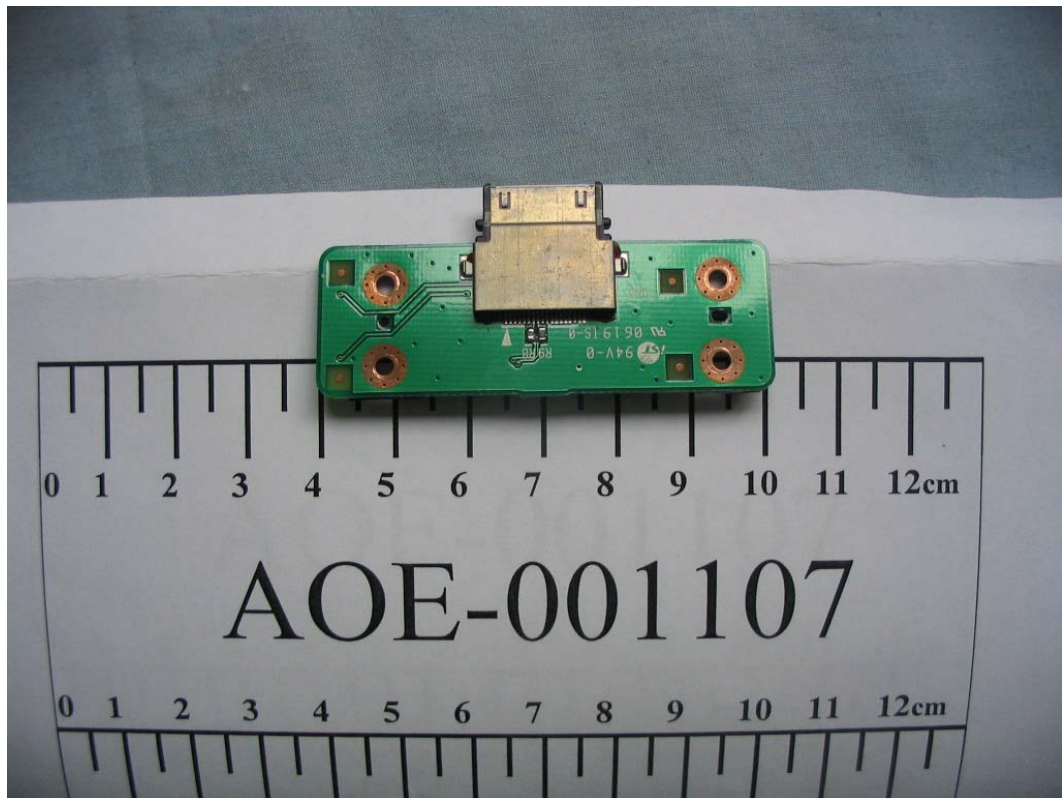
FIGURE 34 WIRELESS POINT OF SALE PDA (M/N: MRT320) CHARGING CRADLE BOARD 2 (SIDE 2)
