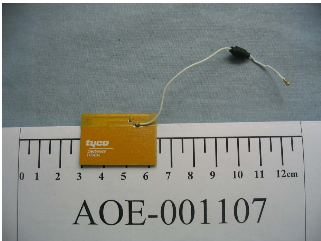
FIGURE 12 WIRELESS POINT OF SALE PDA (M/N: MRT320) HAND-HELD UNIT ANTENNA
