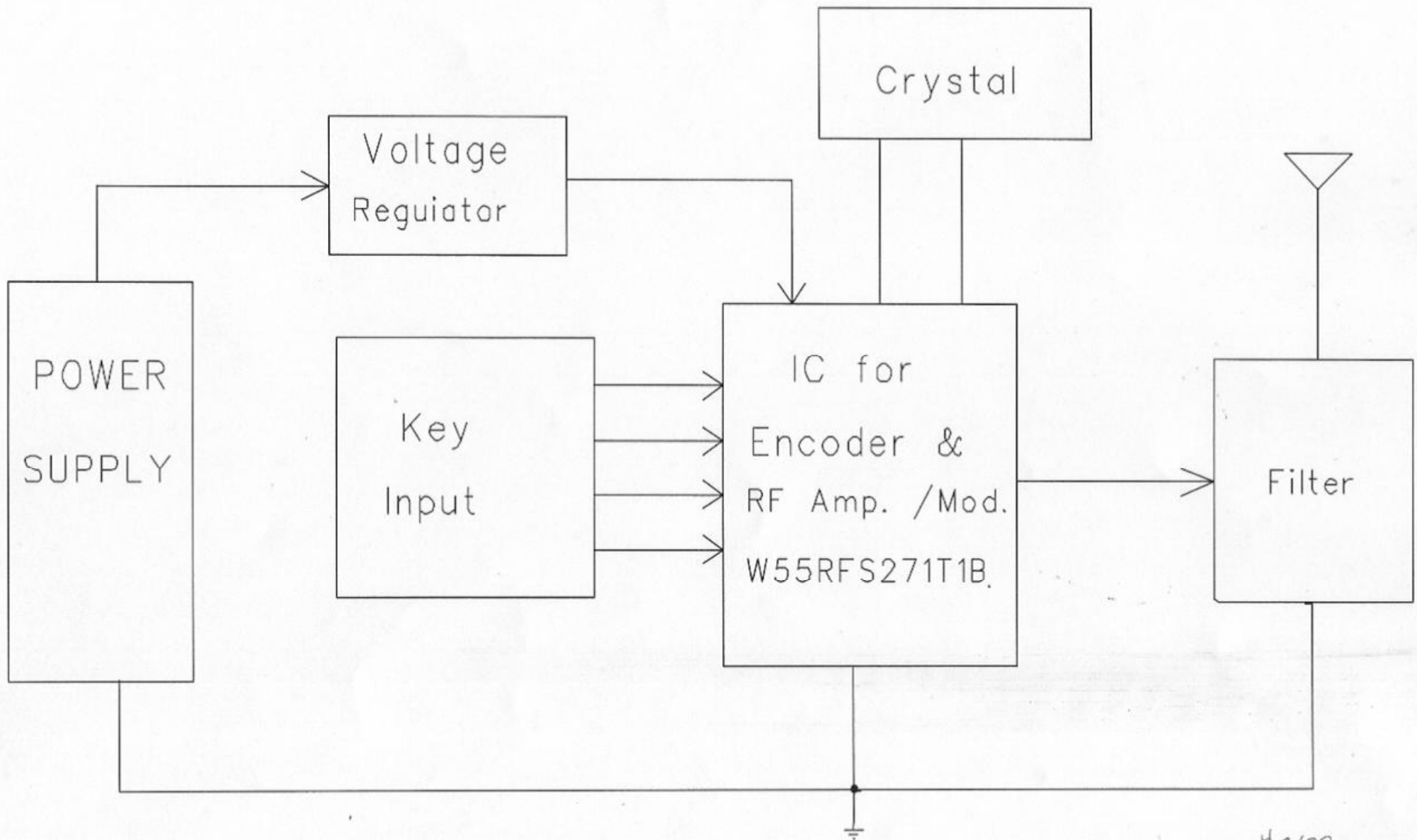
Block Diagram of TX Unit
