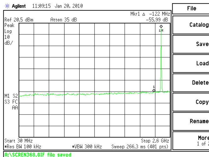
Figure 6.9-5: RF Conducted Spurious Emissions – Mid Channel
