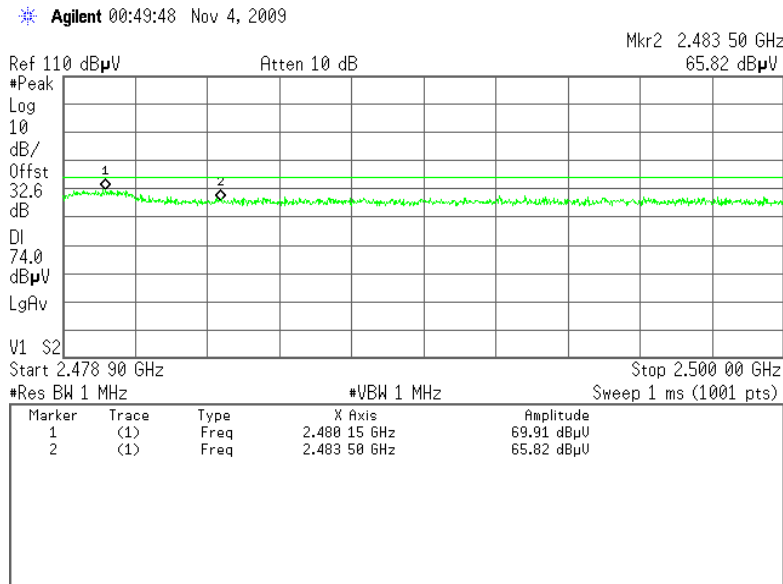
Figure 6.5-1: Restricted Band Starting at 2483.5 MHz (Radiated Peak)
