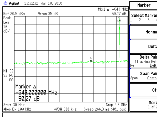
Figure 6.9-3: RF Conducted Spurious Emissions – Low Channel
