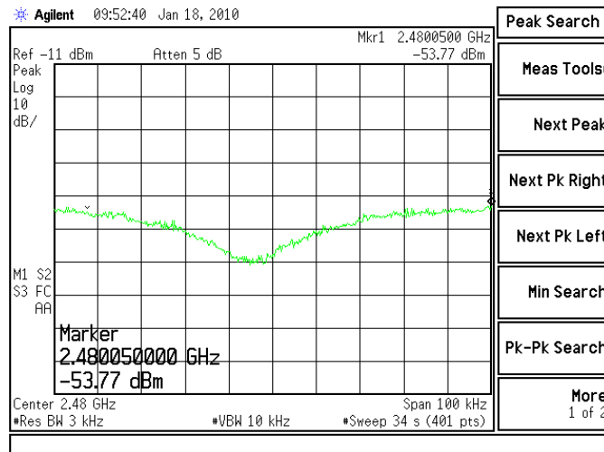
Figure 6.8-3: Power Spectral Density Plot – High Channel
