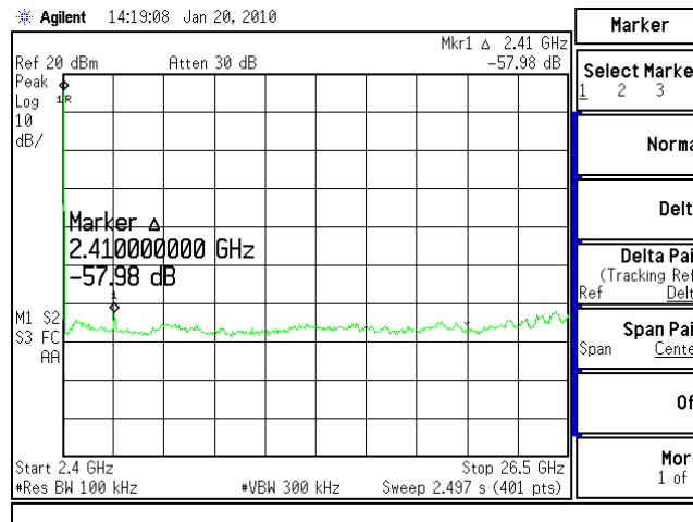
Figure 6.9-6: RF Conducted Spurious Emissions – Mid Channel
