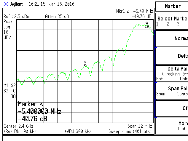
Figure 6.9-1: Lower Band-Edge (Conducted)
