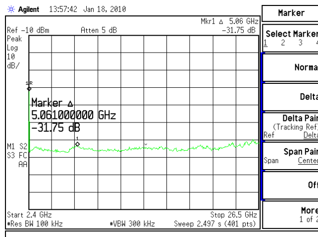
Figure 6.9-8: RF Conducted Spurious Emissions – High Channel
