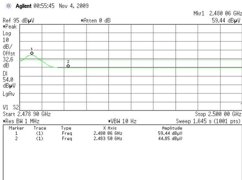
Figure 6.5-2: Restricted Band Starting at 2483.5 MHz (Radiated Average)
