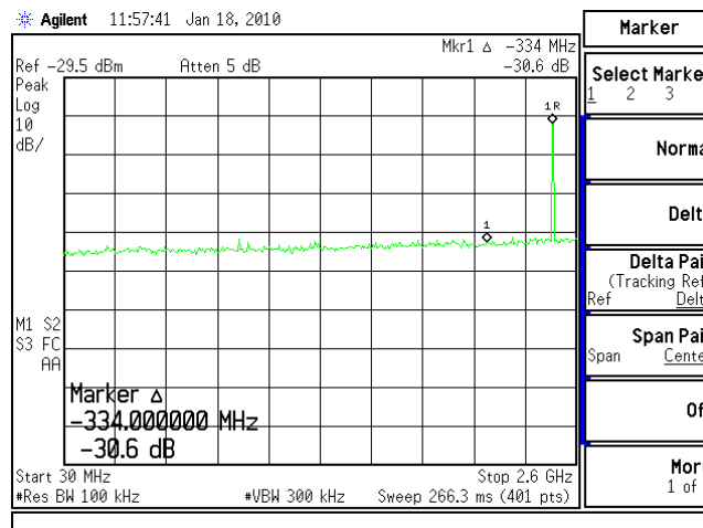
Figure 6.9-7: RF Conducted Spurious Emissions – High Channel
