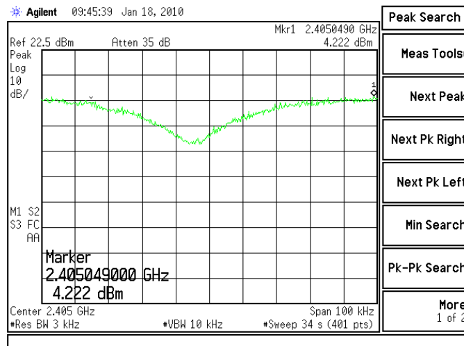
Figure 6.8-1: Power Spectral Density Plot – Low Channel
