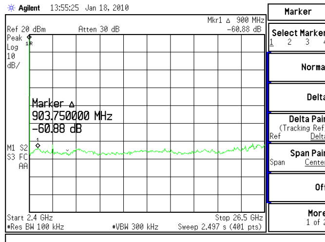
Figure 6.9-4: RF Conducted Spurious Emissions – Low Channel
