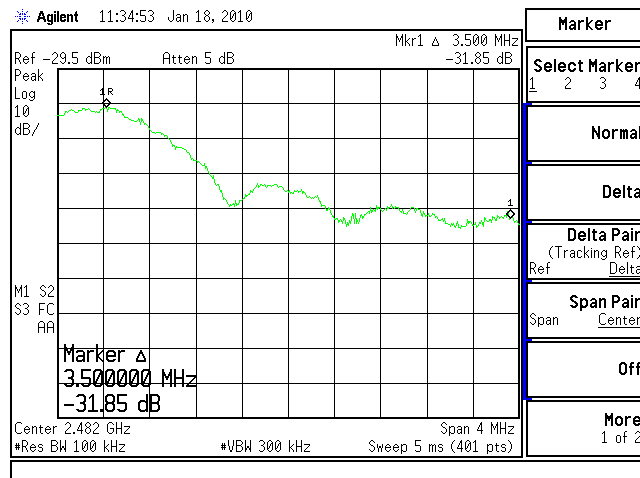
Figure 6.9-2: Upper Band-Edge (Conducted)
