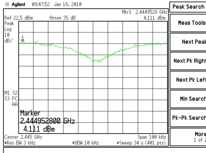
Figure 6.8-2: Power Spectral Density Plot – Mid Channel
