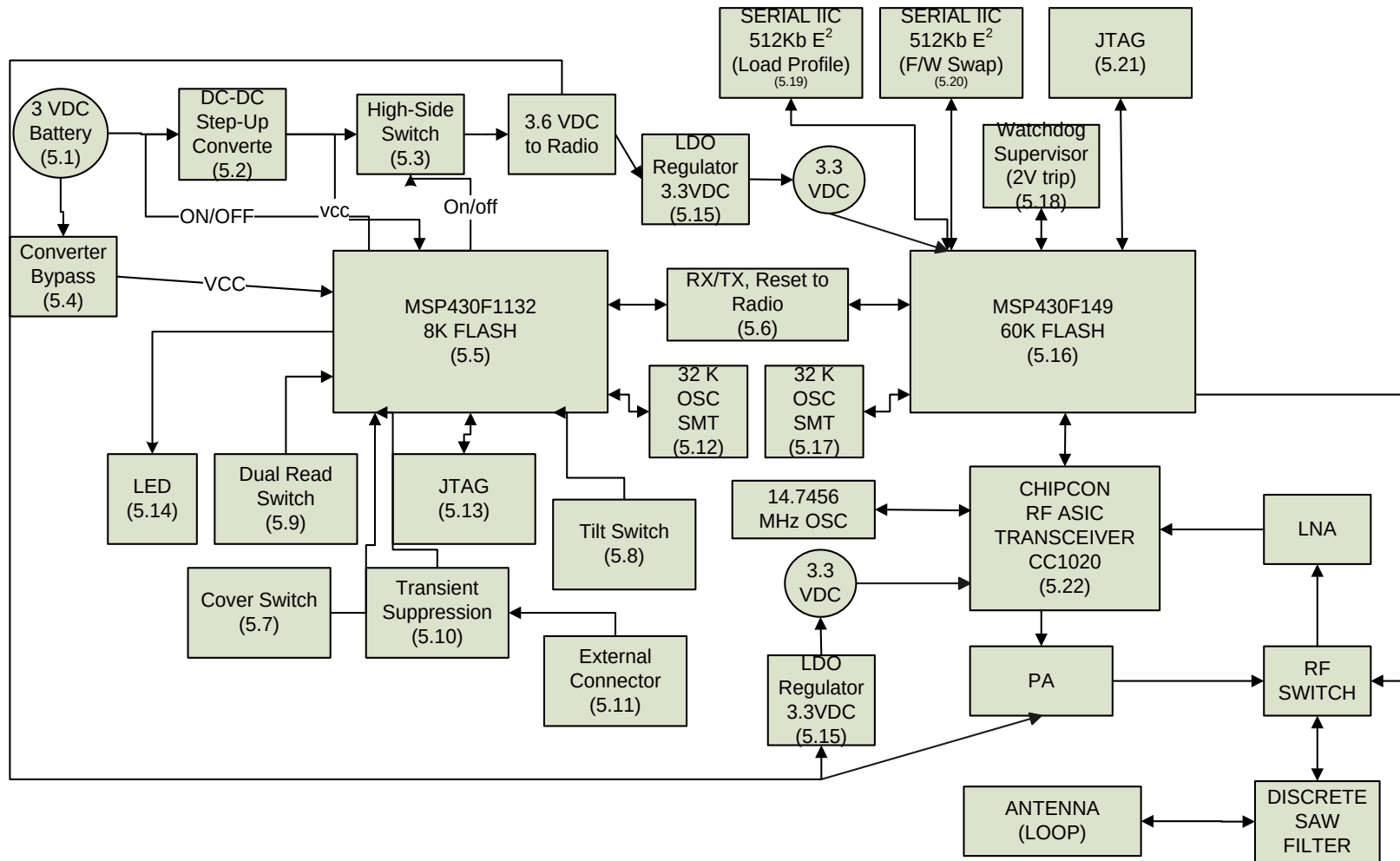
Block Diagram for TEB-HUNTSS710, FASY-0710-0003/0004
