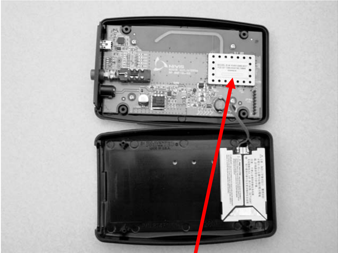
-Interior of NetLINC Transceiver
