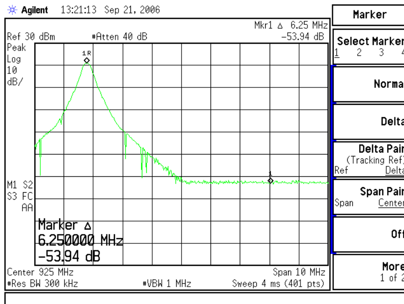
Figure 6.8.1-2: Upper Band-Edge
