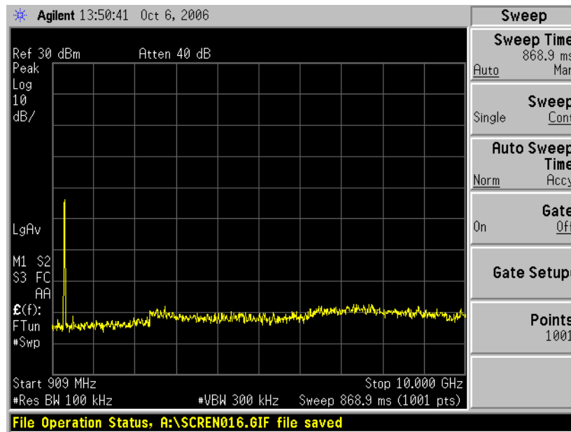
Figure 6.8.2-2: RF Conducted Spurious Emissions – Low Channel
