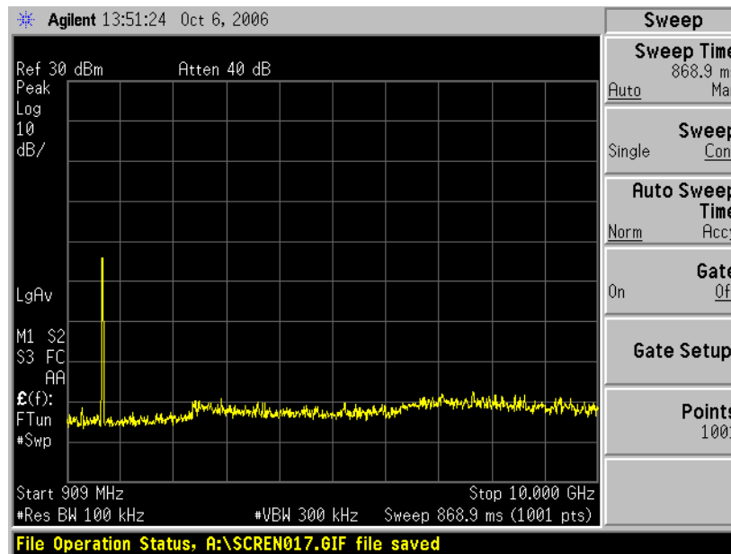
Figure 6.8.2-6: RF Conducted Spurious Emissions – High Channel
