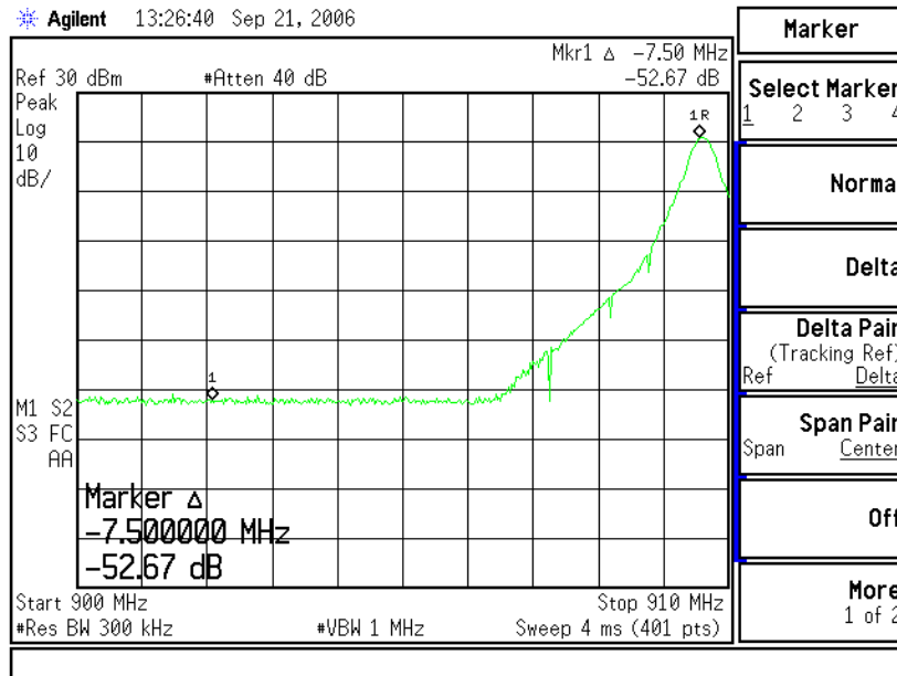
Figure 6.8.1-1: Lower Band-Edge
