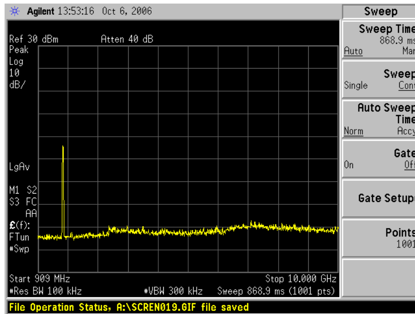
Figure 6.8.2-4: RF Conducted Spurious Emissions – Mid Channel
